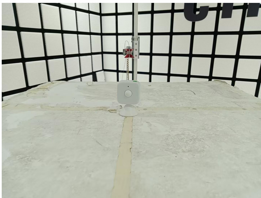
Radiated spurious emission Test Setup-2(1GHz-18GHz)
