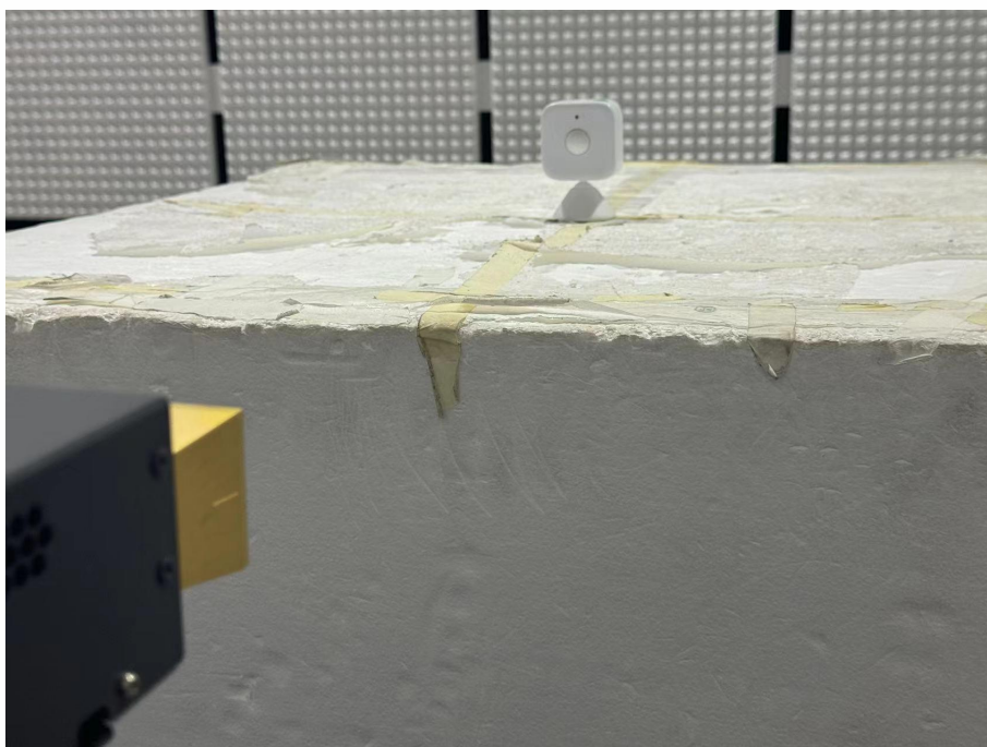
Radiated spurious emission Test Setup-4(Above 41GHz)
