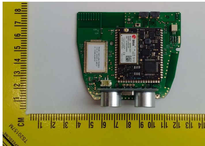
Figure 1: Top Side
