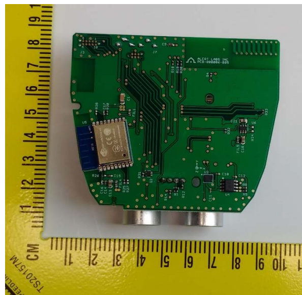
Figure 2: Bottom Side
