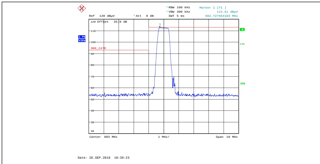
Plot 5.2.4.2.1. Band-Edge Radiated Emissions, Lower Band-edge Rx Antenna in Vertical Polarization, 903.0 MHz
