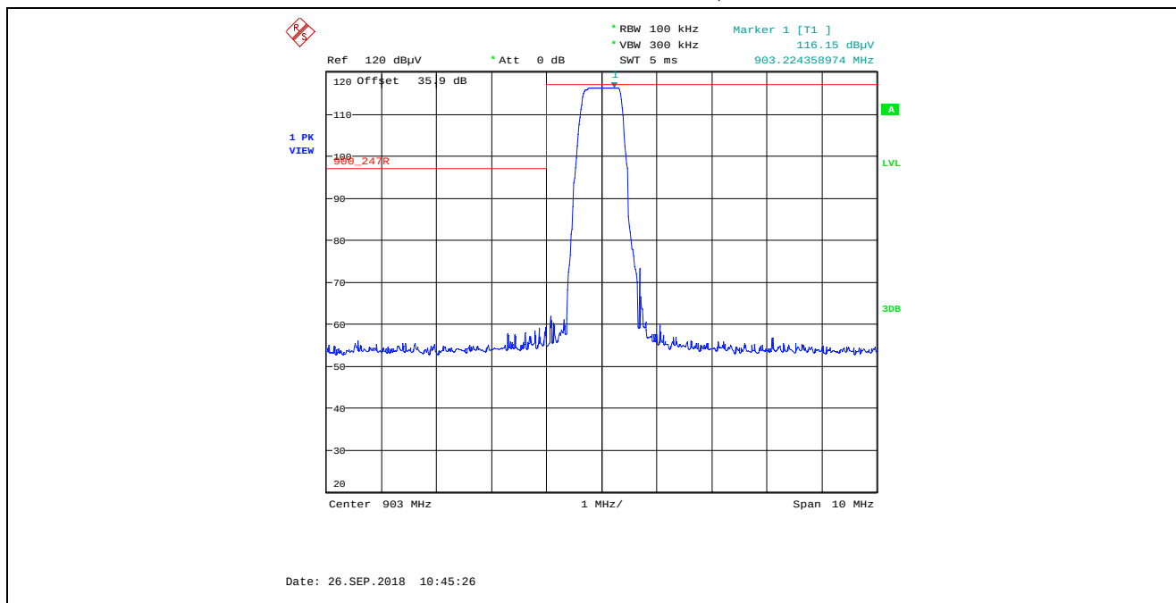
Plot 5.2.4.2.2. Band-Edge Radiated Emissions, Lower Band-edge Rx Antenna in Horizontal Polarization, 903.0 MHz
