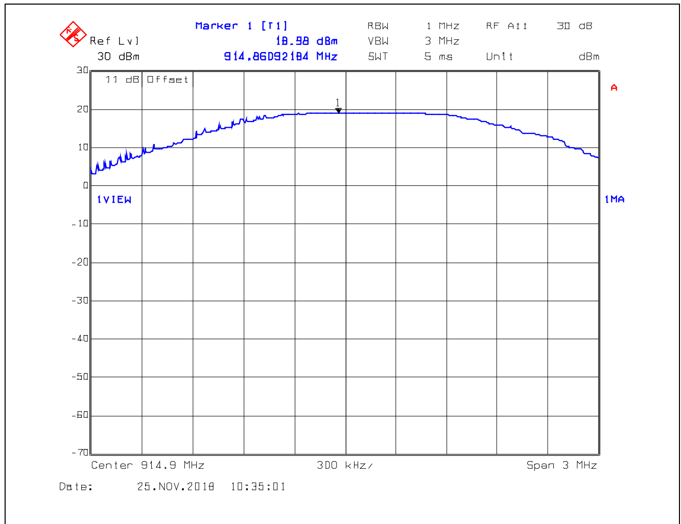
Plot 5.1.4.2. Maximum Peak Conducted Output Power, 914.9 MHz
