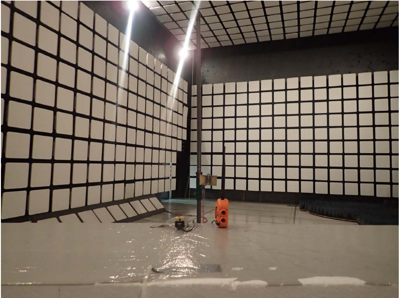
Radiated Emissions @ 3 m, Orthogonal Position 2 EUT in Host Device (Alert Labs Sumpie Sump Pump Monitor)
