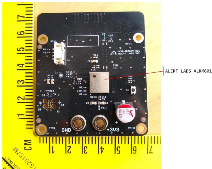
Figure 1: ALRM001 embedded on test PCB
