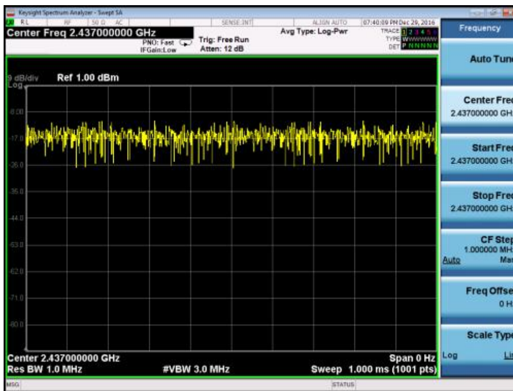
Test plot of Duty Cycle for 802.11n -HT20
