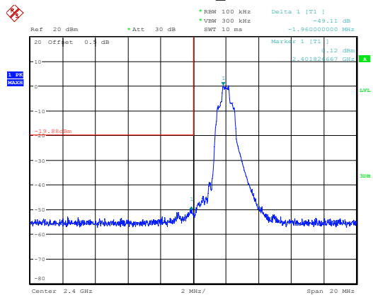
3DH1_Low
