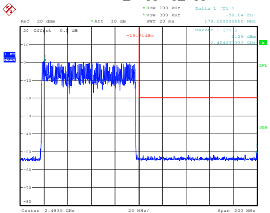
3DH1_Hopping_Upper
