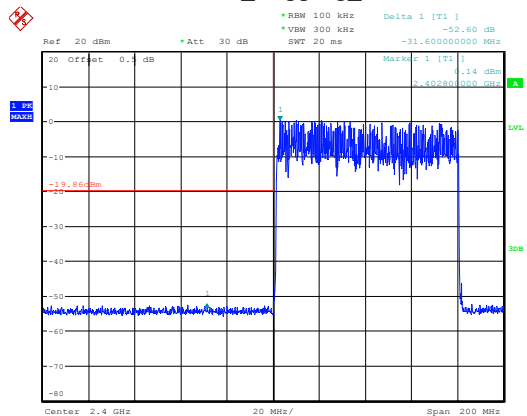
3DH1_Hopping_Lower
