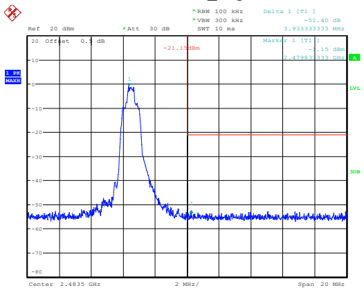
3DH1_High
