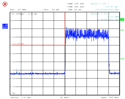
2DH1_Hopping_Lower
