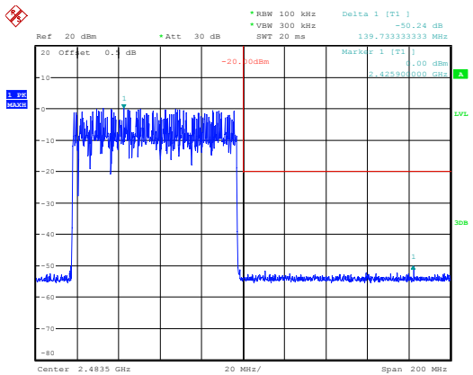
2DH1_Hopping_Upper
