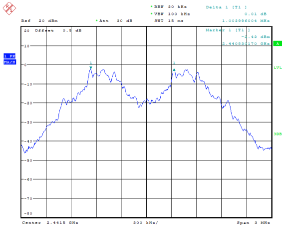
GFSK_Middle 1.004 MHz
