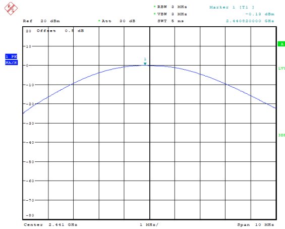
GFSK_Middle -0.13 dBm
