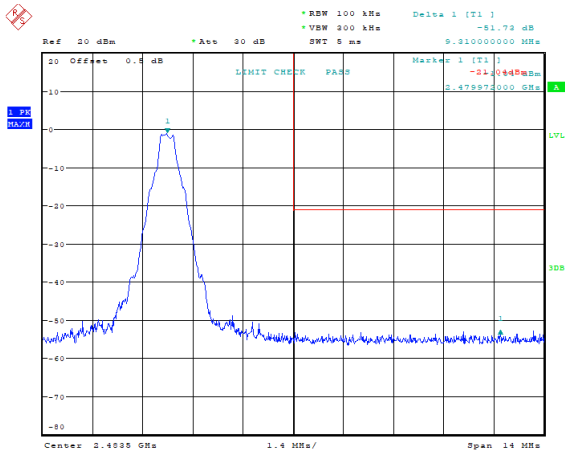
GFSK_High 51.73 dB
