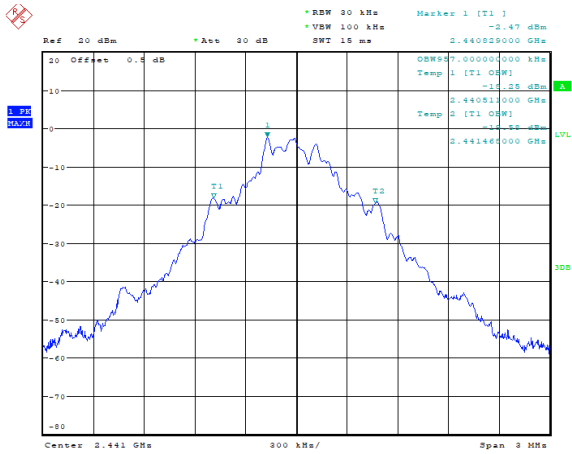
GFSK_Middle 0.957 MHz
