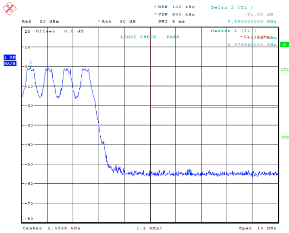
GFSK_Hopping_Upper 51.88 dB
