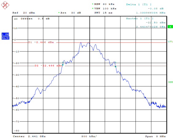
GFSK_Middle 1.034 MHz
