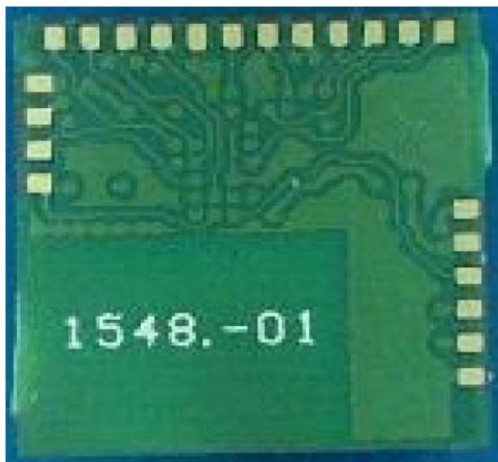
EUT – Bottom View
