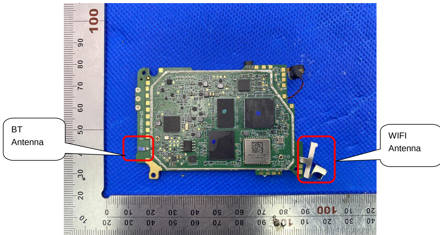
INTERNAL VIEW OF EUT (FIGURE 4)
