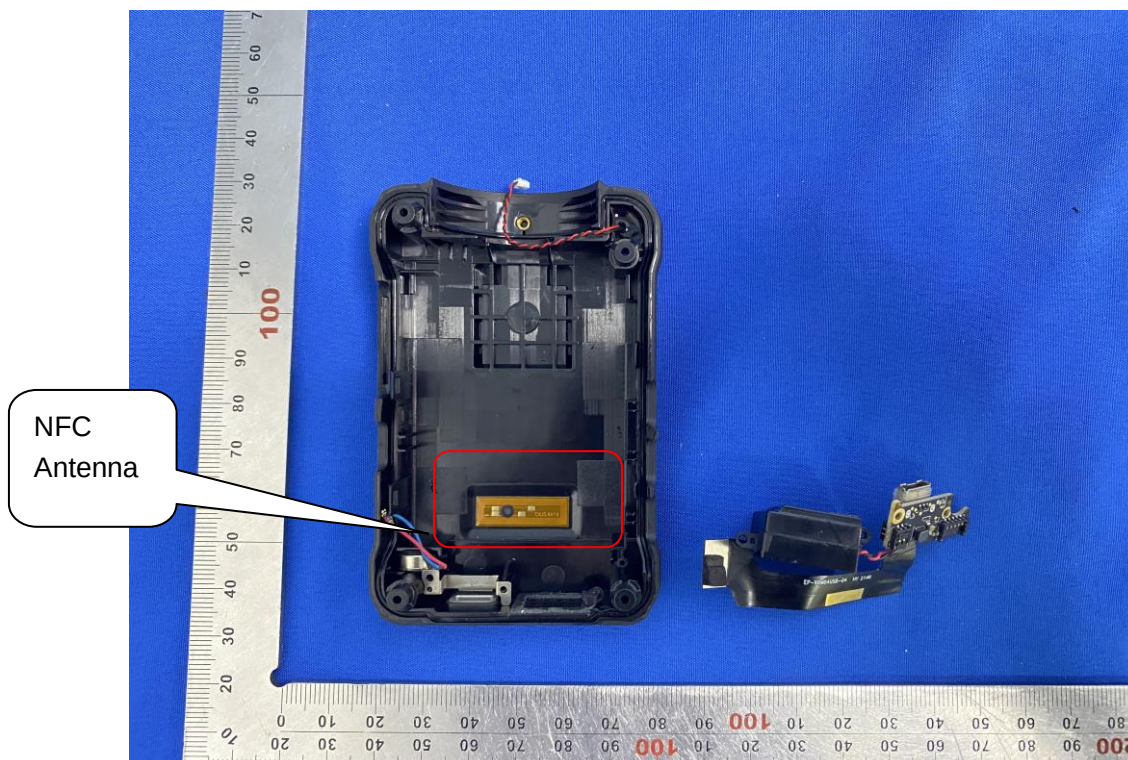
OPEN VIEW OF EUT (FIGURE 4)
