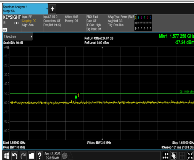
Band14-5MHz-QPSK-23305-1RB#0-Range3:1559~1610MHz
