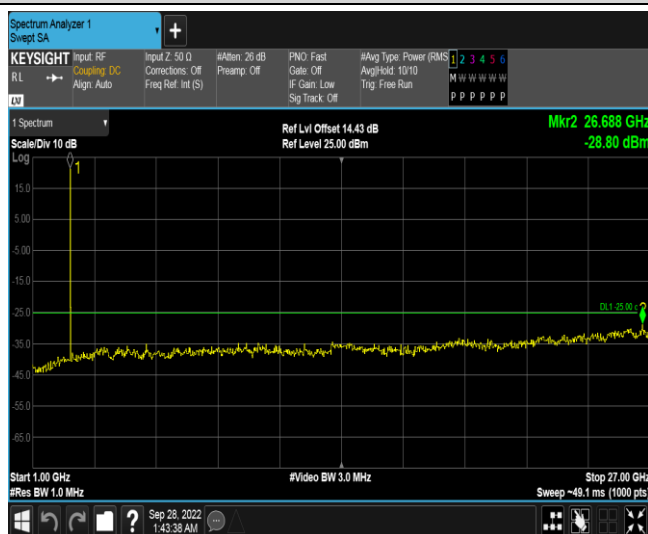
Band41-15MHz-16QAM-40620-1RB#0-Range2:1000~27000MHz
