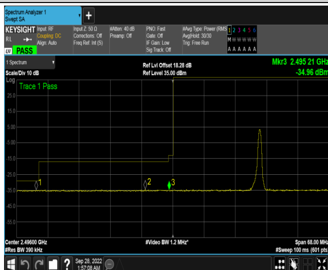
Band41-20MHz-QPSK-39750-100RB#0
