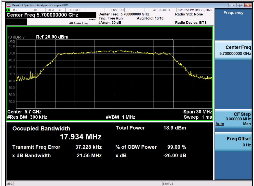
Test_Graph_802.11ac20_Chain A_5700_MCS0_OBW
