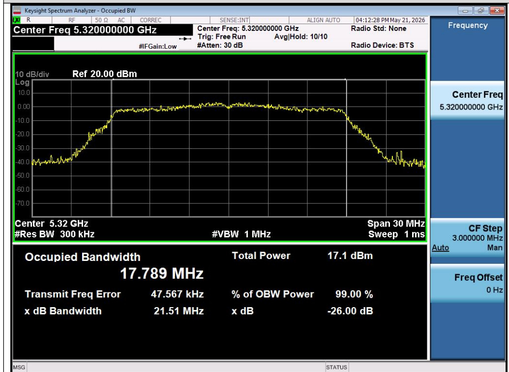
Test_Graph_802.11n20_Chain A_5320_MCS0_OBW
