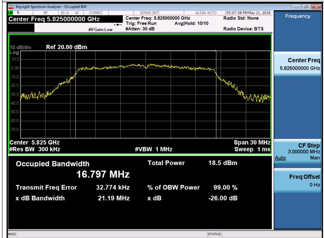
Test_Graph_802.11a_Chain A_5825_6Mbps_OBW
