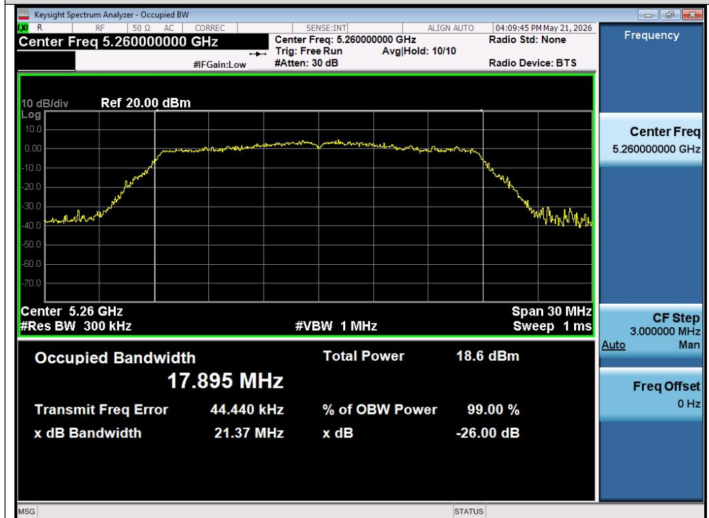
Test_Graph_802.11n20_Chain A_5260_MCS0_OBW
