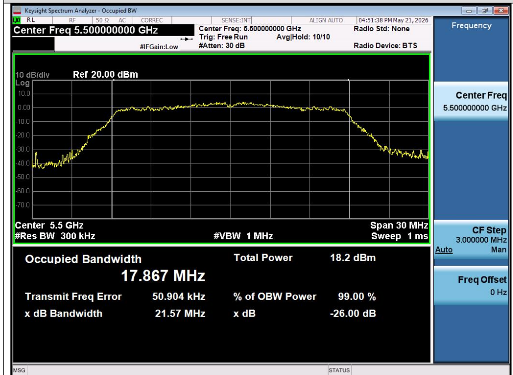
Test_Graph_802.11ac20_Chain A_5500_MCS0_OBW
