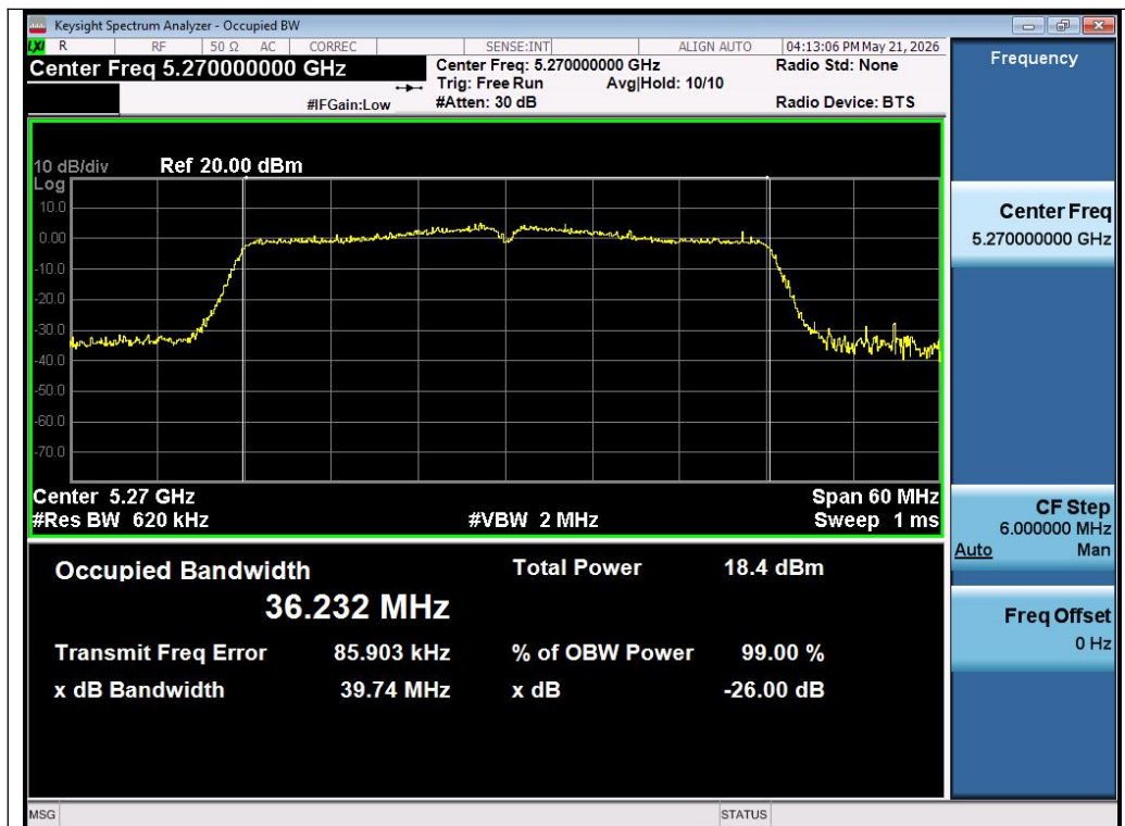
Test_Graph_802.11n40_Chain A_5270_MCS0_OBW
