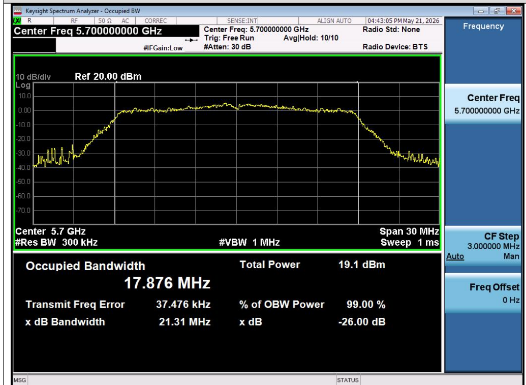
Test_Graph_802.11n20_Chain A_5700_MCS0_OBW
