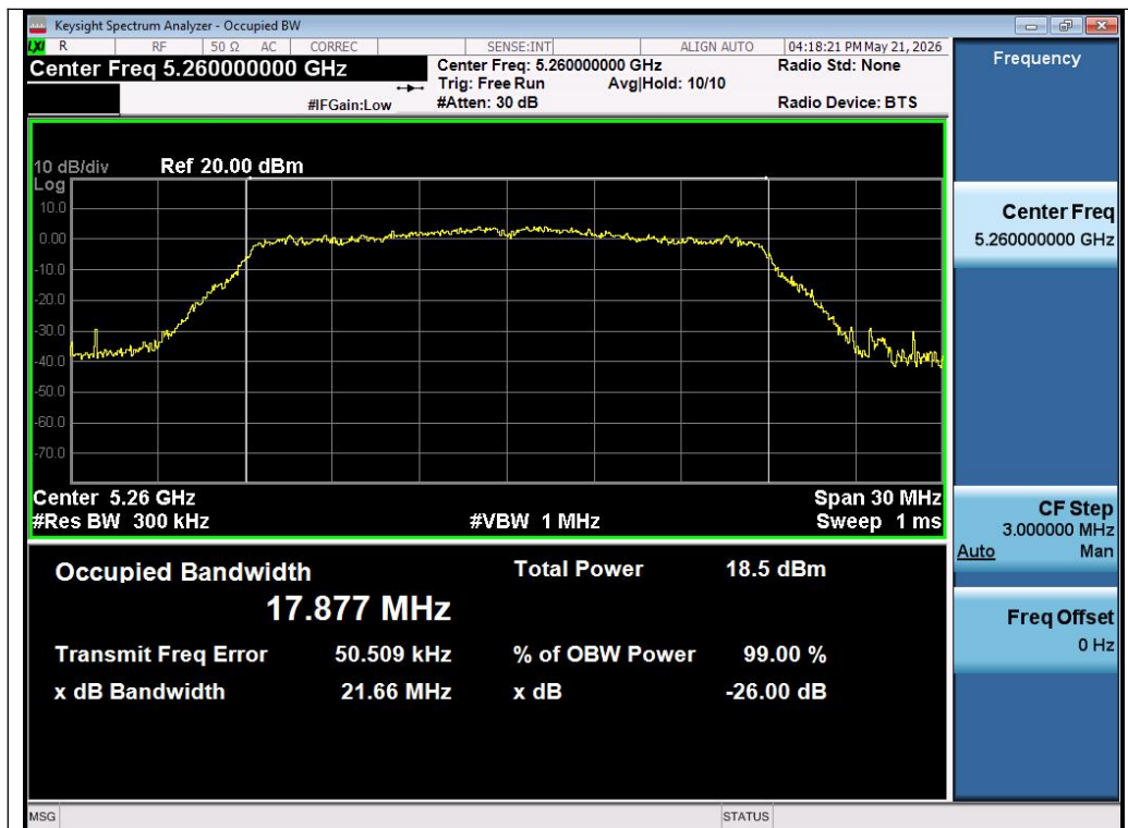
Test_Graph_802.11ac20_Chain A_5260_MCS0_OBW
