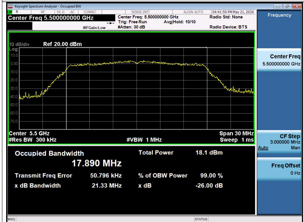
Test_Graph_802.11n20_Chain A_5500_MCS0_OBW
