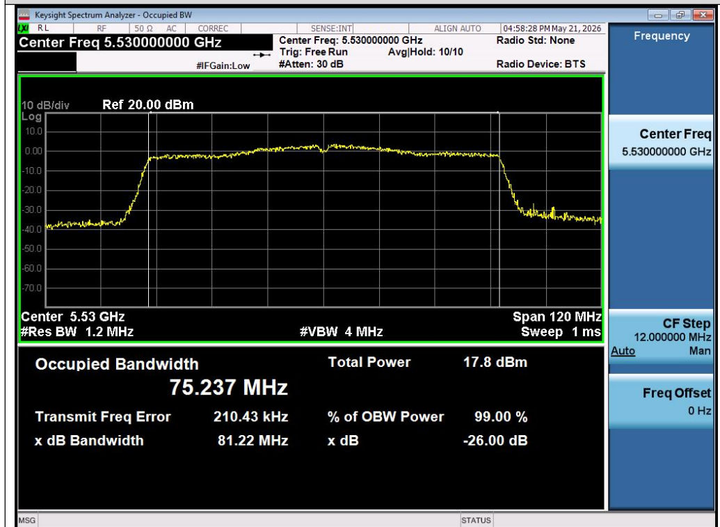
Test_Graph_802.11ac80_Chain A_5530_MCS0_OBW
