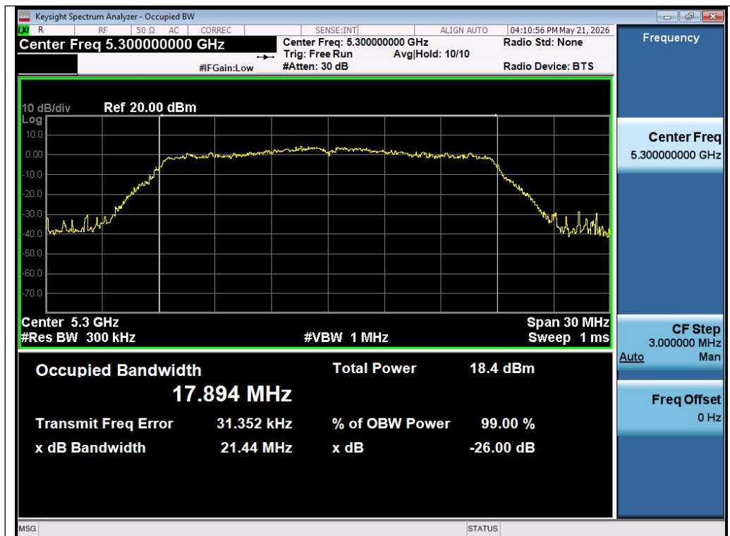
Test_Graph_802.11n20_Chain A_5300_MCS0_OBW
