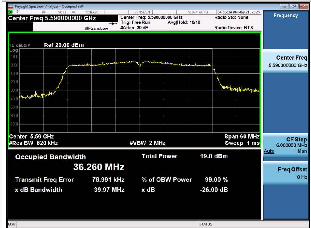
Test_Graph_802.11ac40_Chain A_5590_MCS0_OBW
