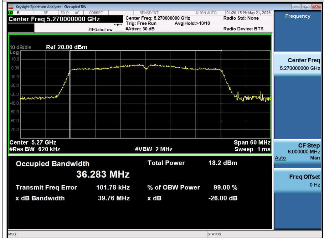
Test_Graph_802.11ac40_Chain A_5270_MCS0_OBW
