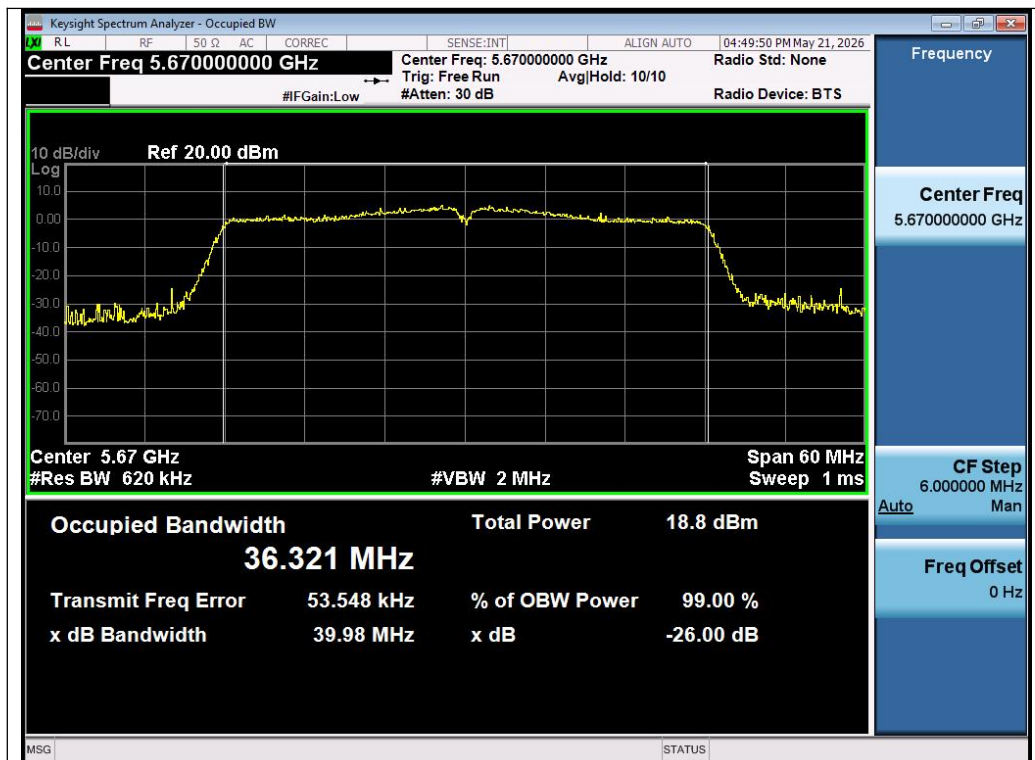
Test_Graph_802.11n40_Chain A_5670_MCS0_OBW
