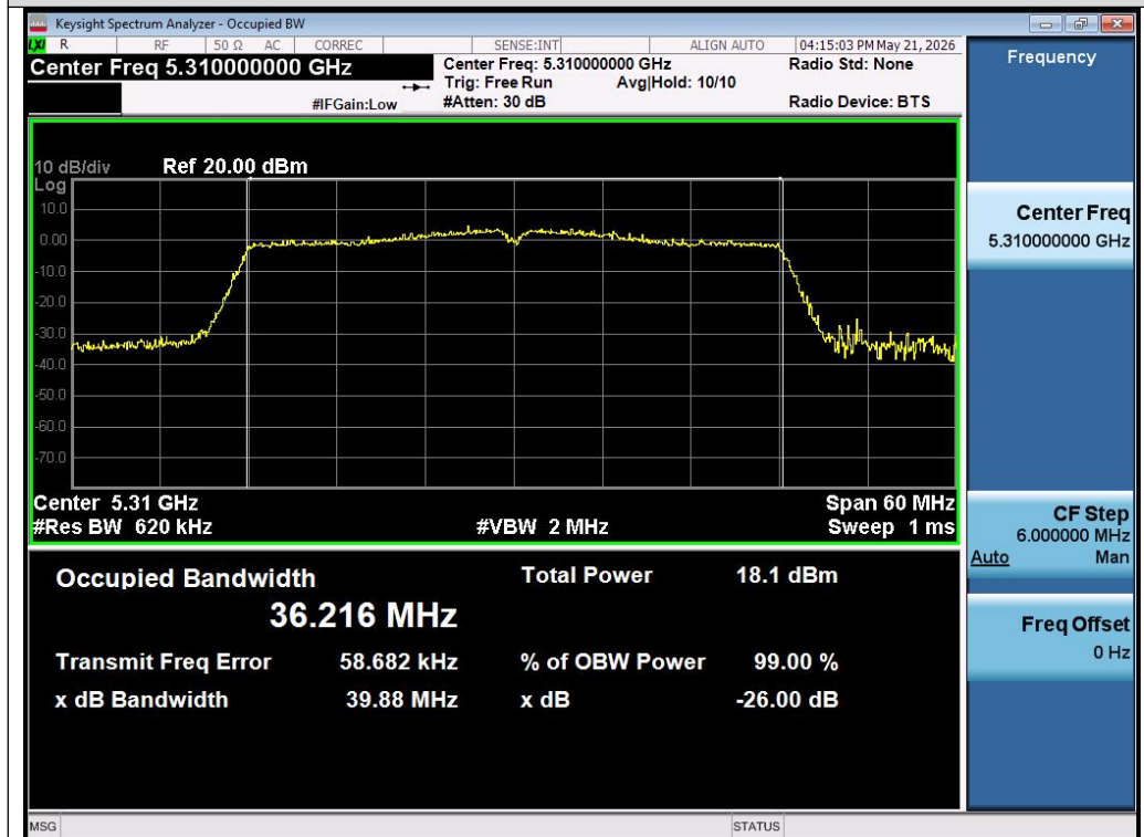
Test_Graph_802.11n40_Chain A_5310_MCS0_OBW
