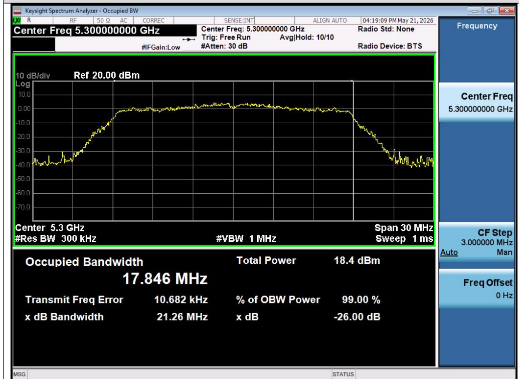
Test_Graph_802.11ac20_Chain A_5300_MCS0_OBW
