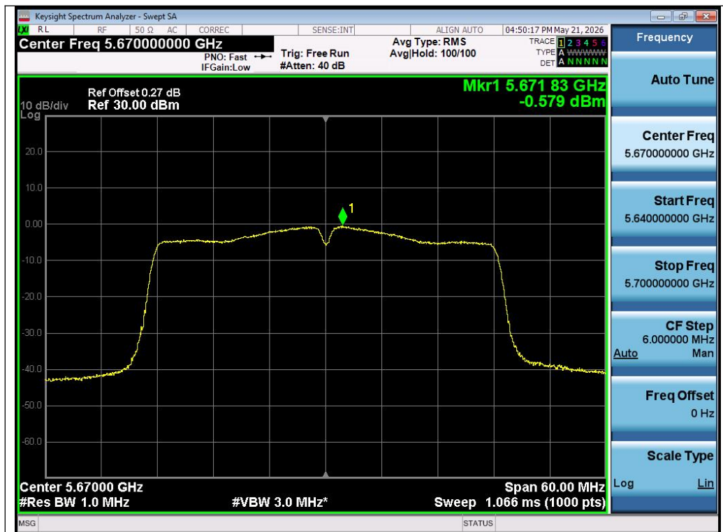
Test_Graph_802.11n40_Chain A_5670_MCS0_PSD
