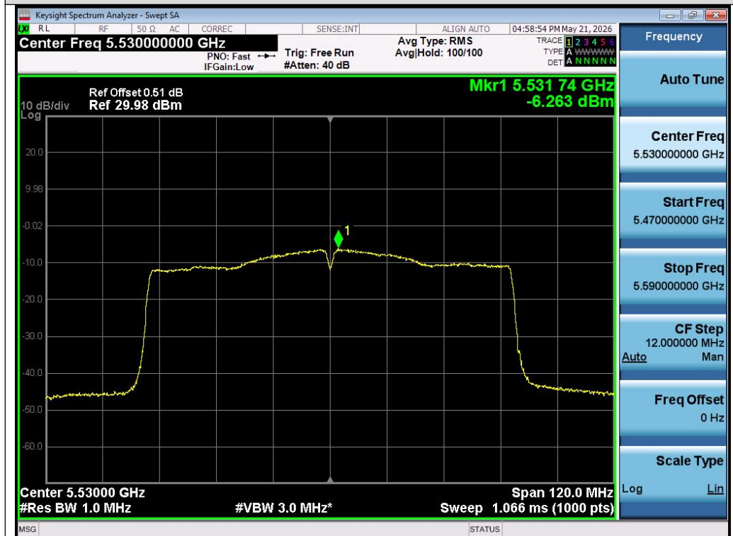
Test_Graph_802.11ac80_Chain A_5530_MCS0_PSD
