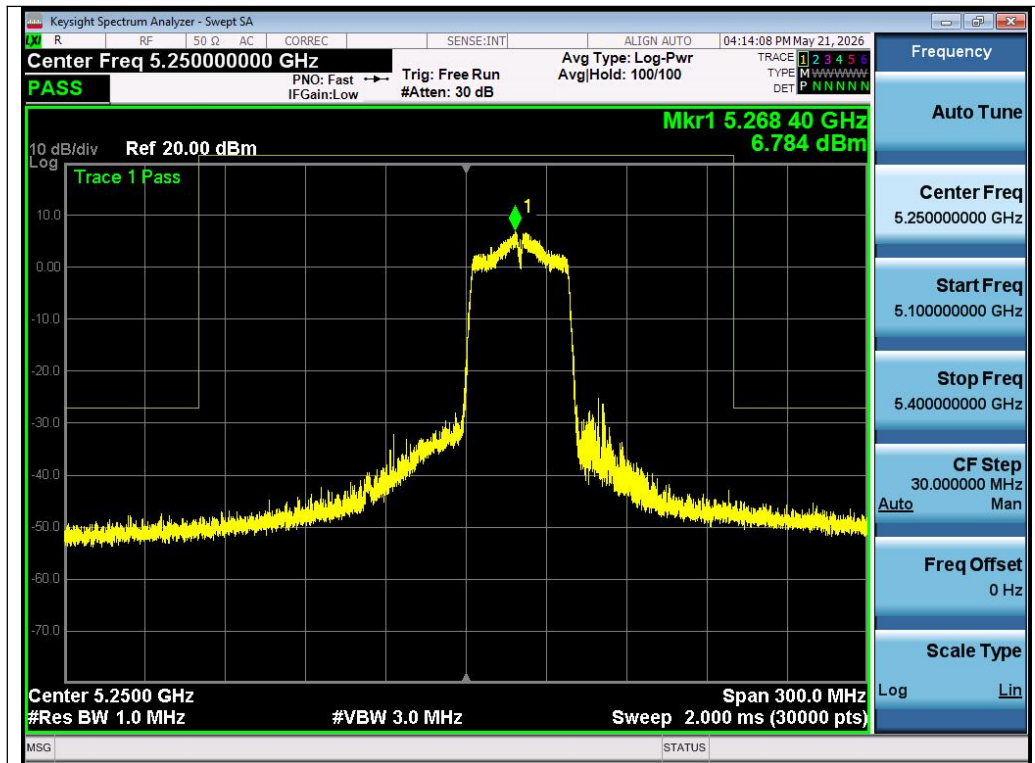
Test_Graph_802.11n40_Chain A_5270_MCS0_Frequency Band 3
