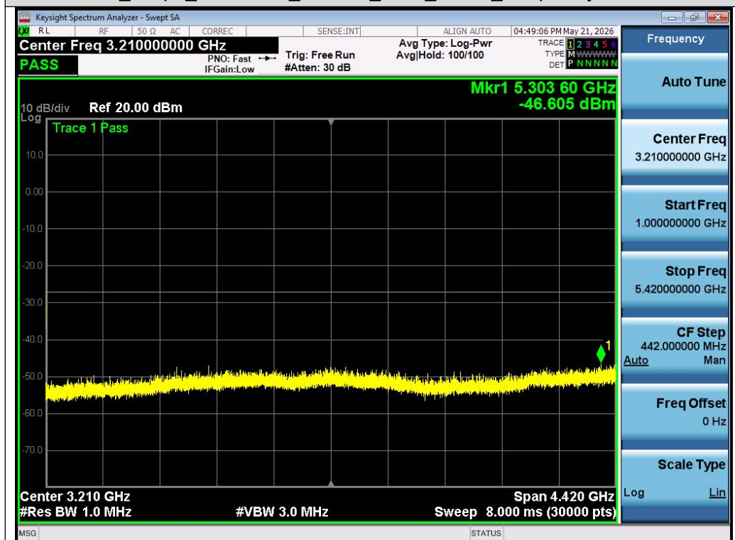
Test_Graph_802.11n40_Chain A_5590_MCS0_Frequency Band 2
