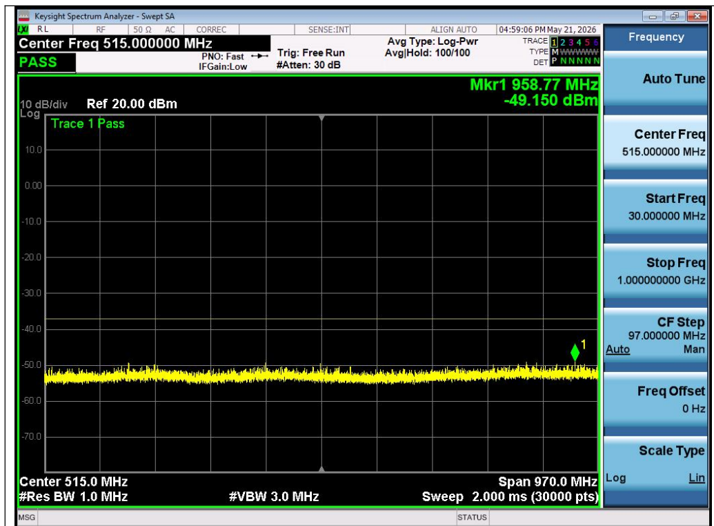
Test_Graph_802.11ac80_Chain A_5530_MCS0_Frequency Band 1
