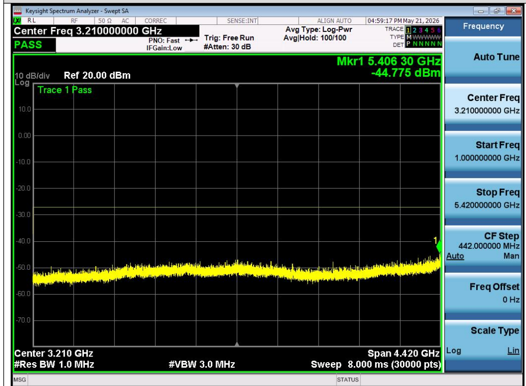
Test_Graph_802.11ac80_Chain A_5530_MCS0_Frequency Band 2
