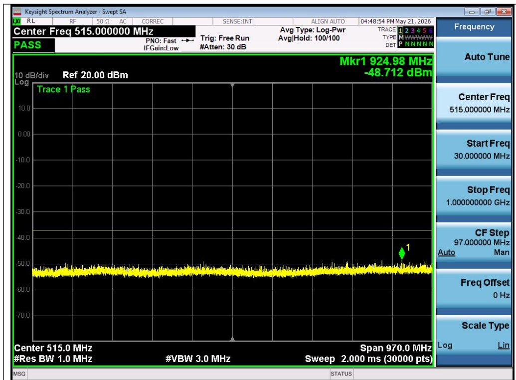
Test_Graph_802.11n40_Chain A_5590_MCS0_Frequency Band 1
