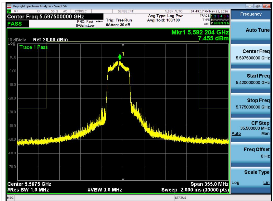
Test_Graph_802.11n40_Chain A_5590_MCS0_Frequency Band 3
