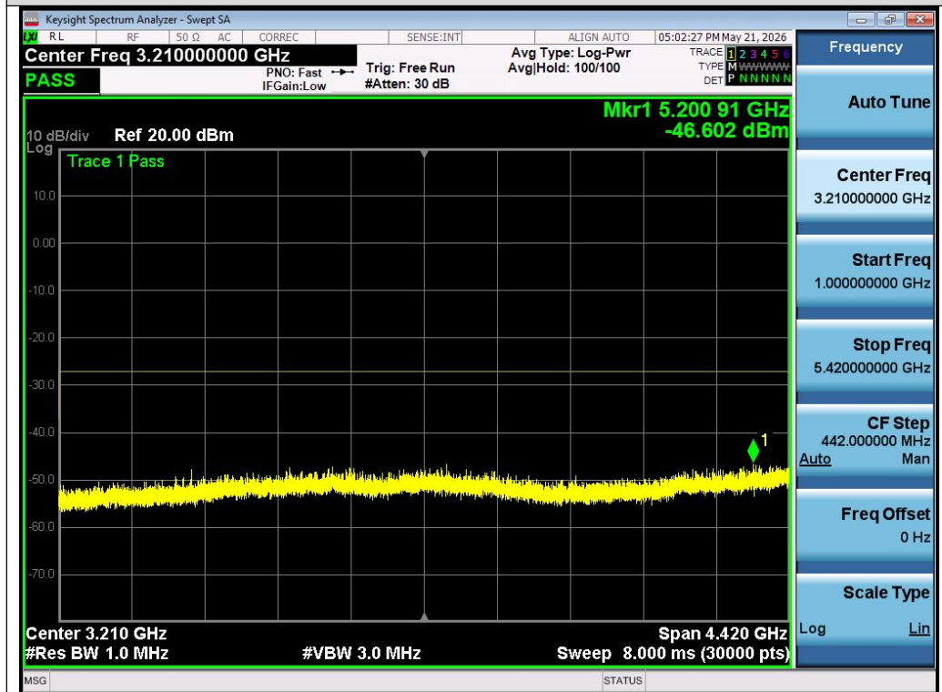
Test_Graph_802.11ac80_Chain A_5610_MCS0_Frequency Band 2
