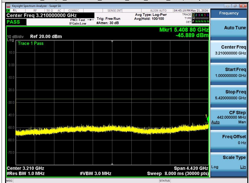
Test_Graph_802.11n40_Chain A_5510_MCS0_Frequency Band 2
