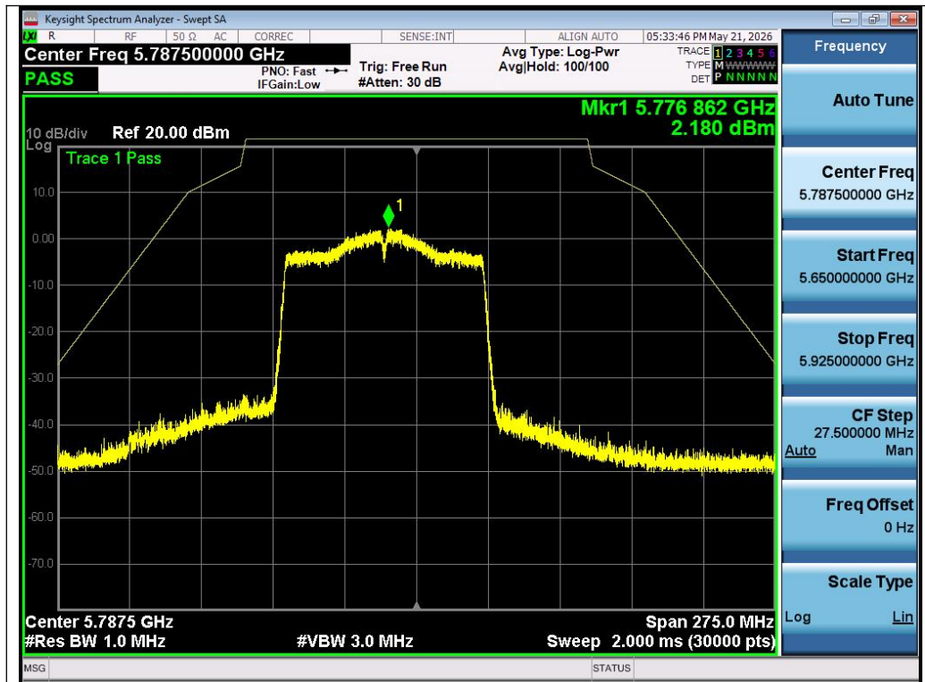
Test_Graph_802.11ac80_Chain A_5775_MCS0_Frequency Band3
