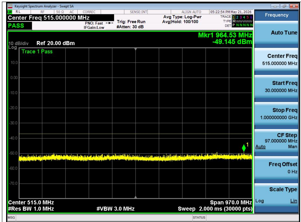
Test_Graph_802.11n40_Chain A_5795_MCS0_Frequency Band1
