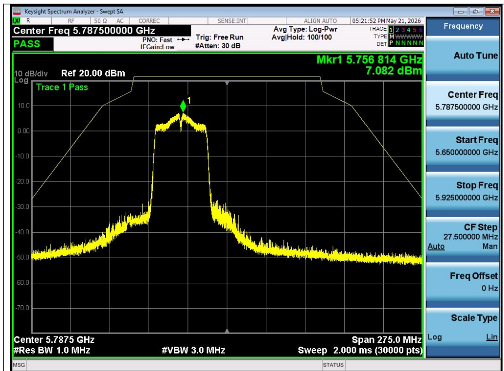
Test_Graph_802.11n40_Chain A_5755_MCS0_Frequency Band3
