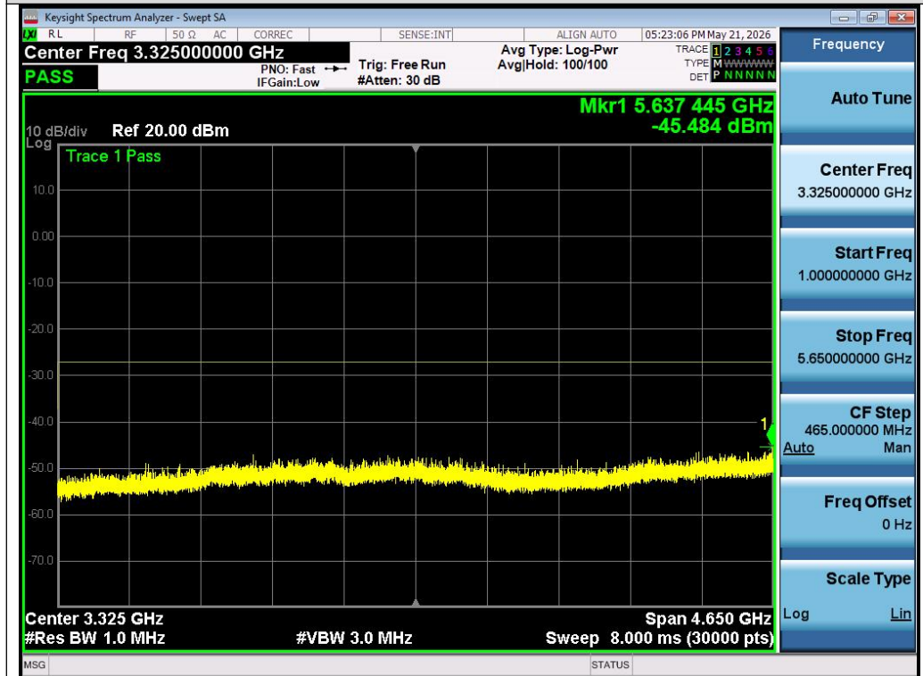
Test_Graph_802.11n40_Chain A_5795_MCS0_Frequency Band2
