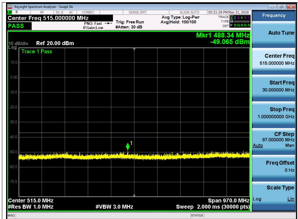
Test_Graph_802.11n40_Chain A_5755_MCS0_Frequency Band1
