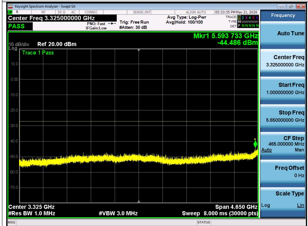
Test_Graph_802.11ac80_Chain A_5775_MCS0_Frequency Band2
