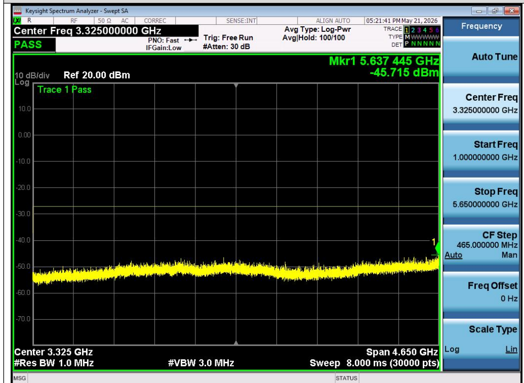
Test_Graph_802.11n40_Chain A_5755_MCS0_Frequency Band2
