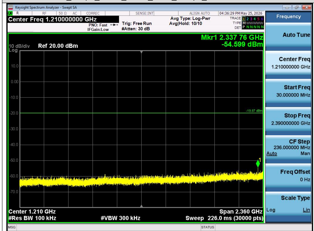
Test Graph LE1M ANT1 2402 1Mbps Lower Band Emissions
