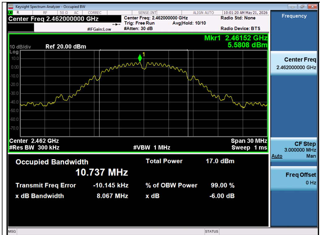
Test_Graph_802.11b_Chain A_2462_1Mbps_DTSBW
