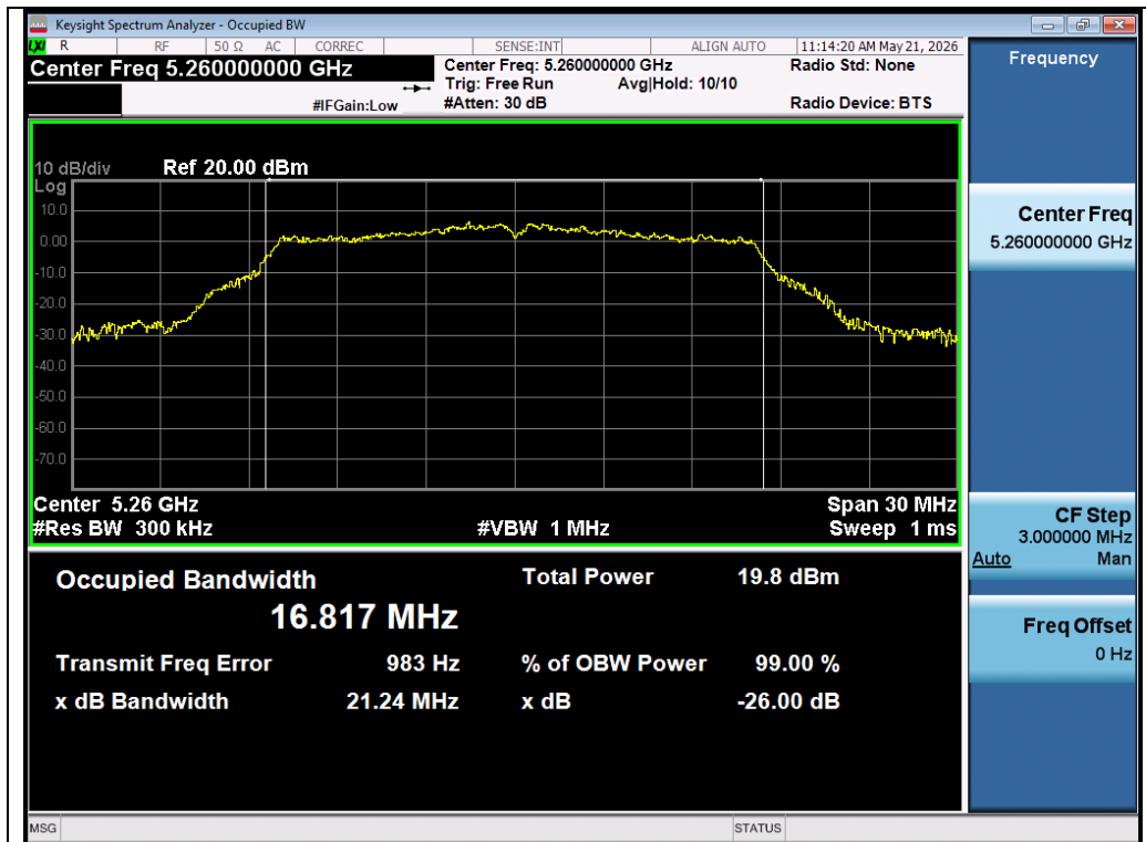
Test_Graph_802.11a_Chain A_5260_6Mbps_OBW
