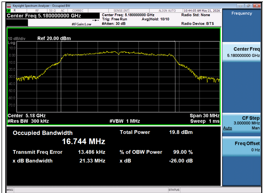
Test_Graph_802.11a_Chain A_5180_6Mbps_OBW
