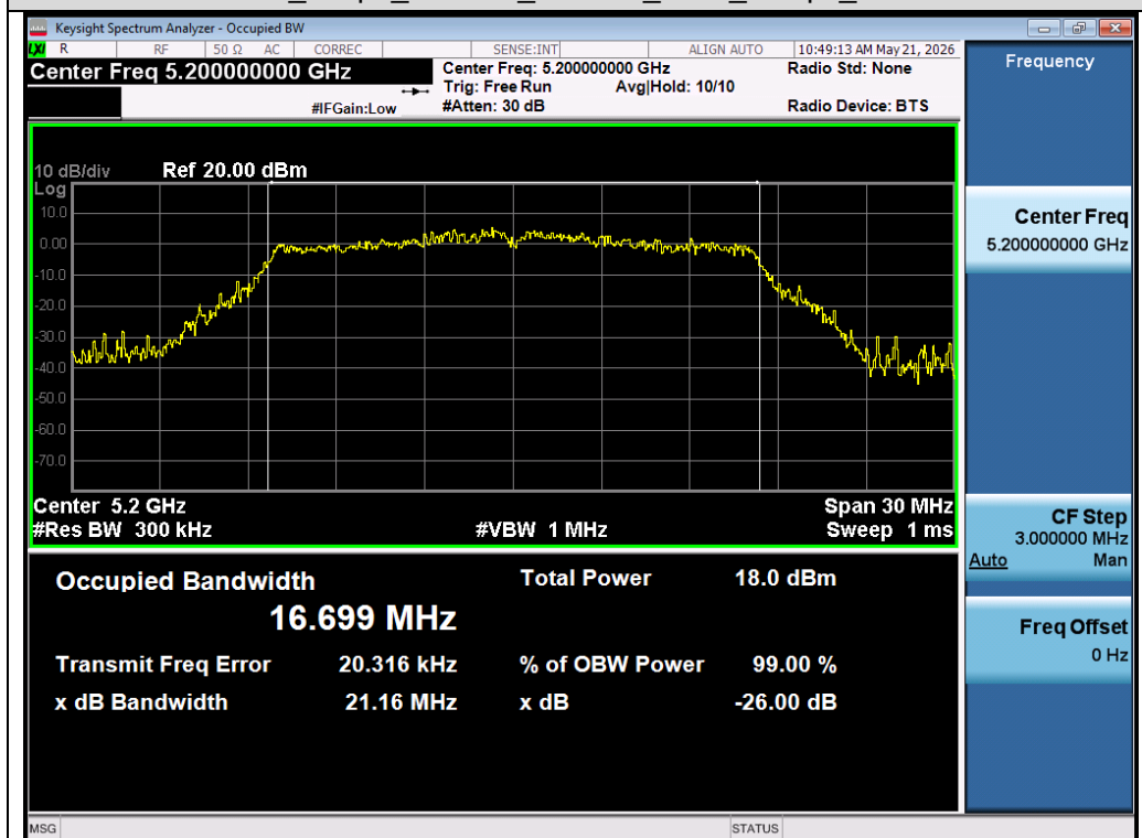
Test_Graph_802.11a_Chain A_5200_6Mbps_OBW
