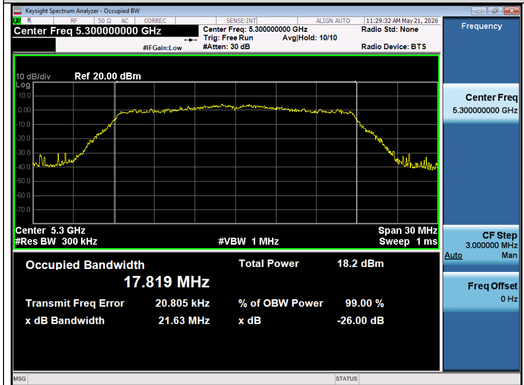
Test_Graph_802.11ac20_Chain A_5300_MCS0_OBW
