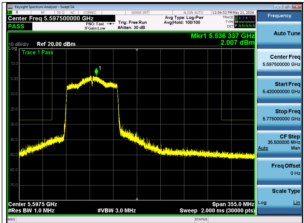
Test_Graph_802.11ac80_Chain A_5530_MCS0_Frequency Band 3
