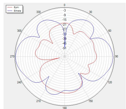
Phi=0 freq=2500MHz
