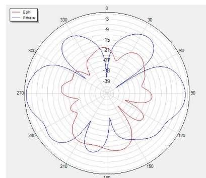
Phi=0 freq=2400MHz
