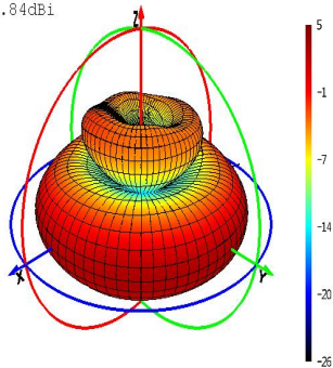
Theta=0 freq=2400MHz
