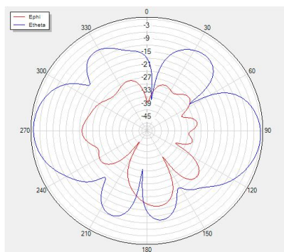
Phi=90 freq=2500MHz
