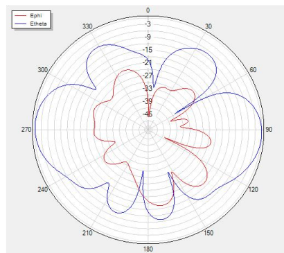
Phi=90 freq=2450MHz
