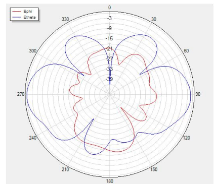
Phi=0 freq=2450MHz
