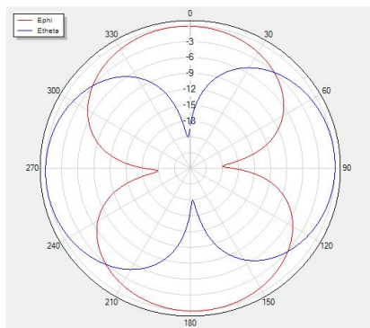
Theta=0 freq=2450MHz
