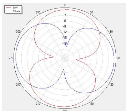
Theta=0 freq=2400MHz
