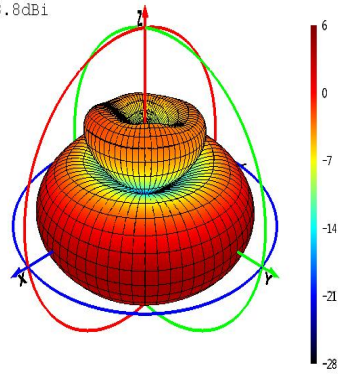
Theta=0 freq=2450MHz
