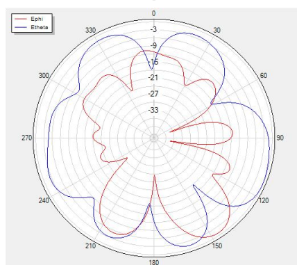
Phi=90 freq=5450MHz
