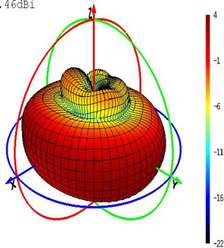
Theta=0 freq=2400MHz
