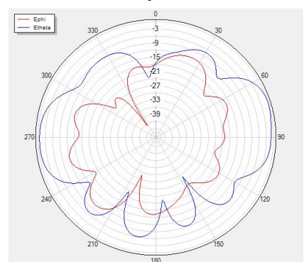
Phi=0 freq=2400MHz
