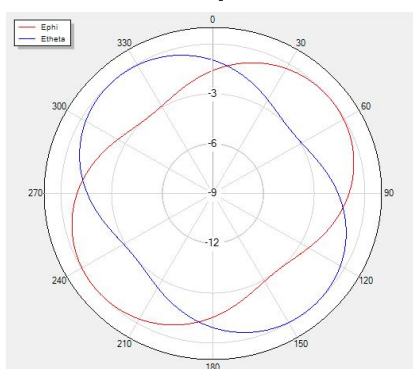
Theta=0 freq=2400MHz
