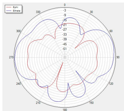
Phi=0 freq=2500MHz
