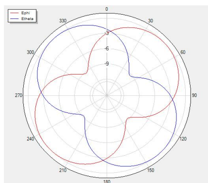
Theta=0 freq=2450MHz
