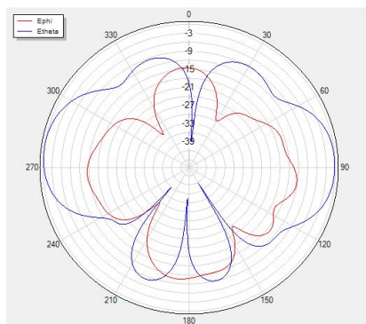
Phi=90 freq=2500MHz
