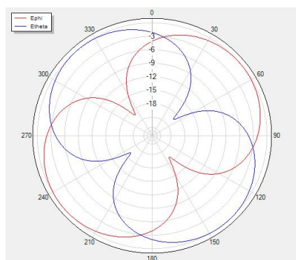
Theta=0 freq=5900MHz
