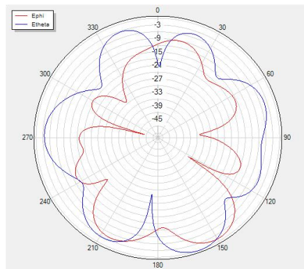
Phi=90 freq=5100MHz
