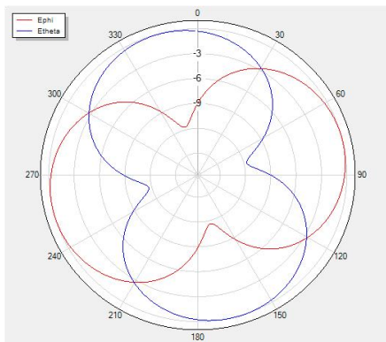
Theta=0 freq=5100MHz
