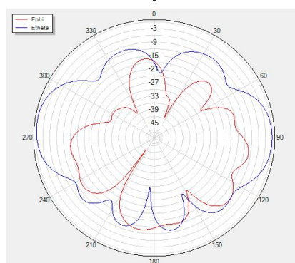
Phi=90 freq=2400MHz
