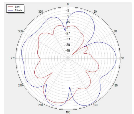
Phi=0 freq=5100MHz
