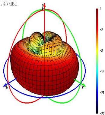
Theta=0 freq=2450MHz
