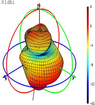
Theta=0 freq=5450MHz
