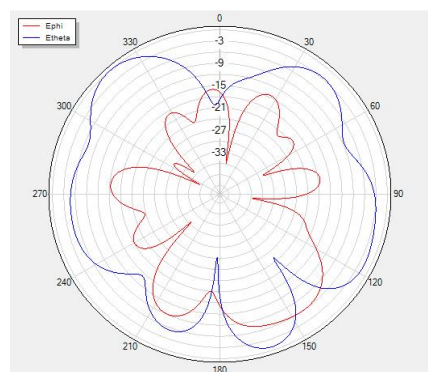
Phi=90 freq=5900MHz
