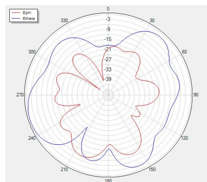
Phi=0 freq=5900MHz
