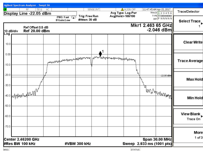
802.11g Chain 1-High channel
