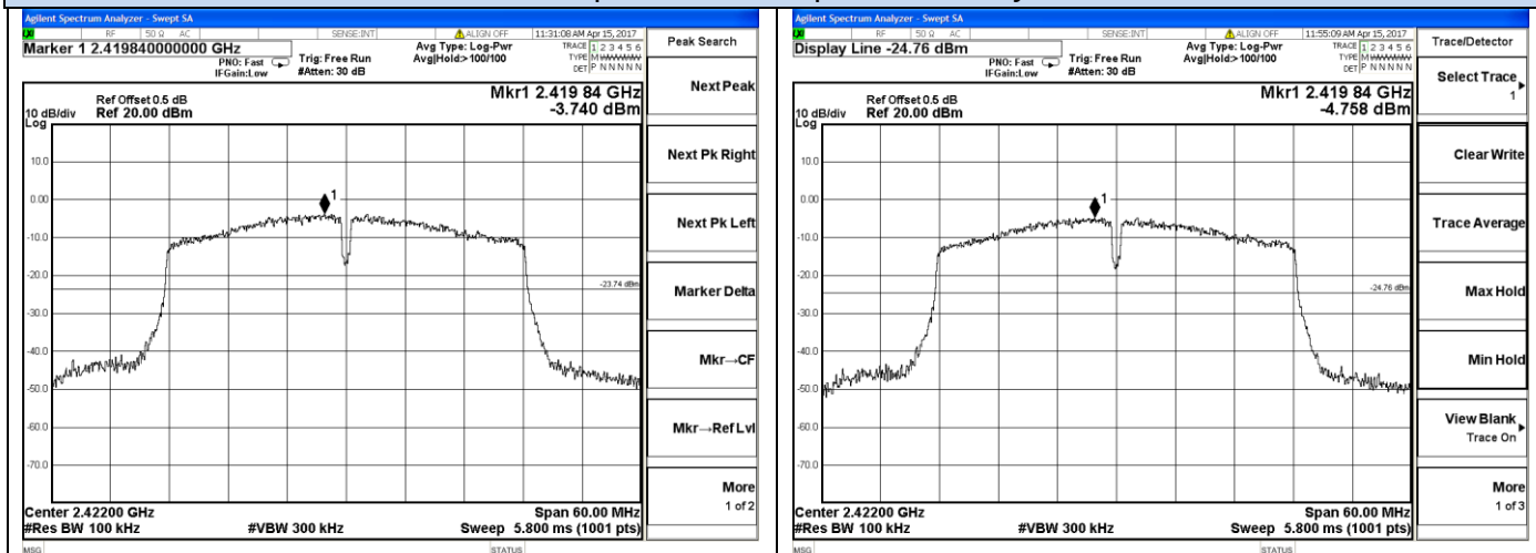
802.11n-HT40 Chain 0-Low channel
