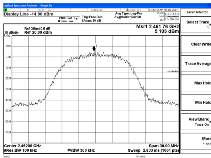
802.11b Chain 1-High channel
