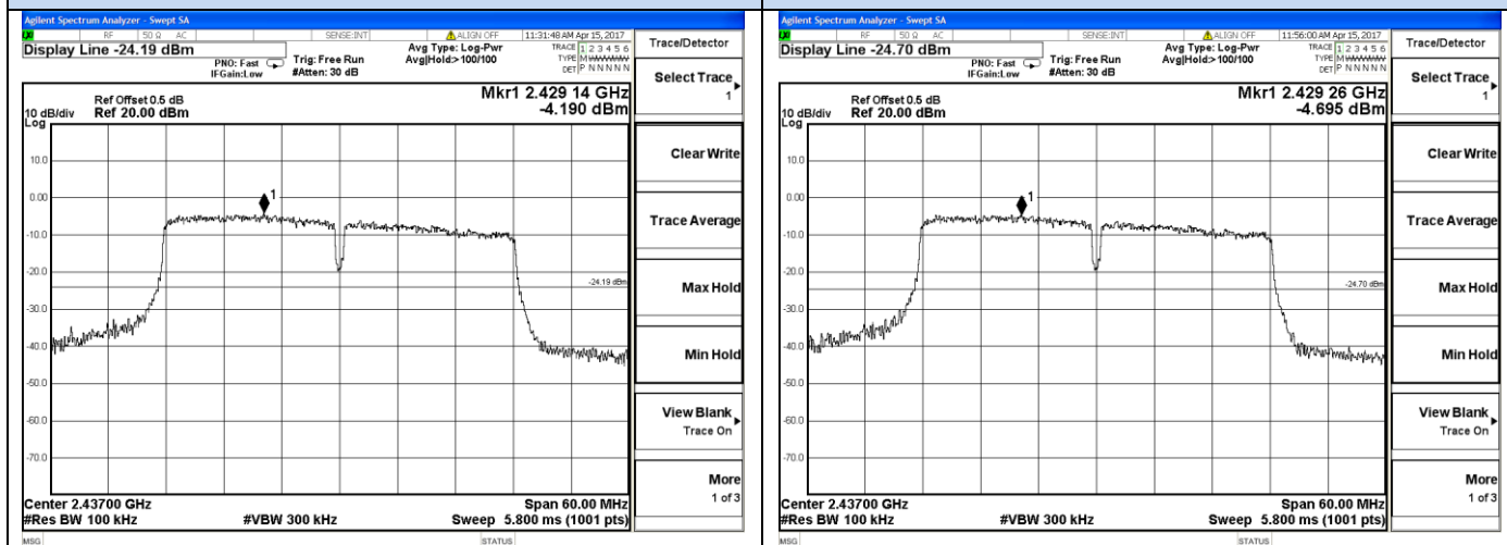
802.11n-HT40 Chain 0-Middle channel
