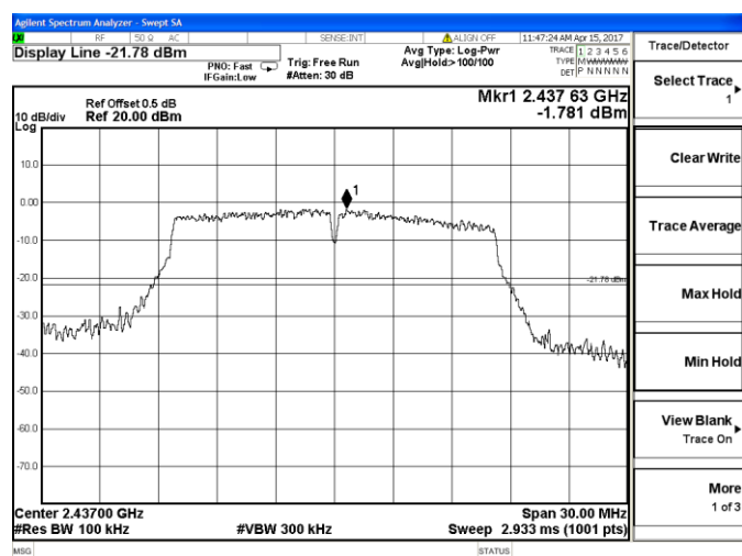
802.11g Chain 1-Middle channel
