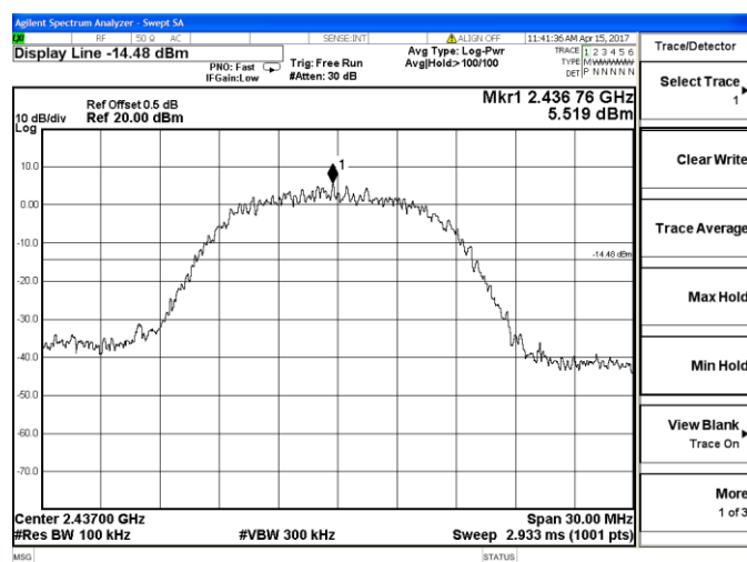
802.11b Chain 1-Middle channel
