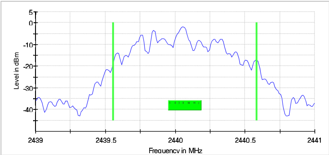
99 % Bandwidth
