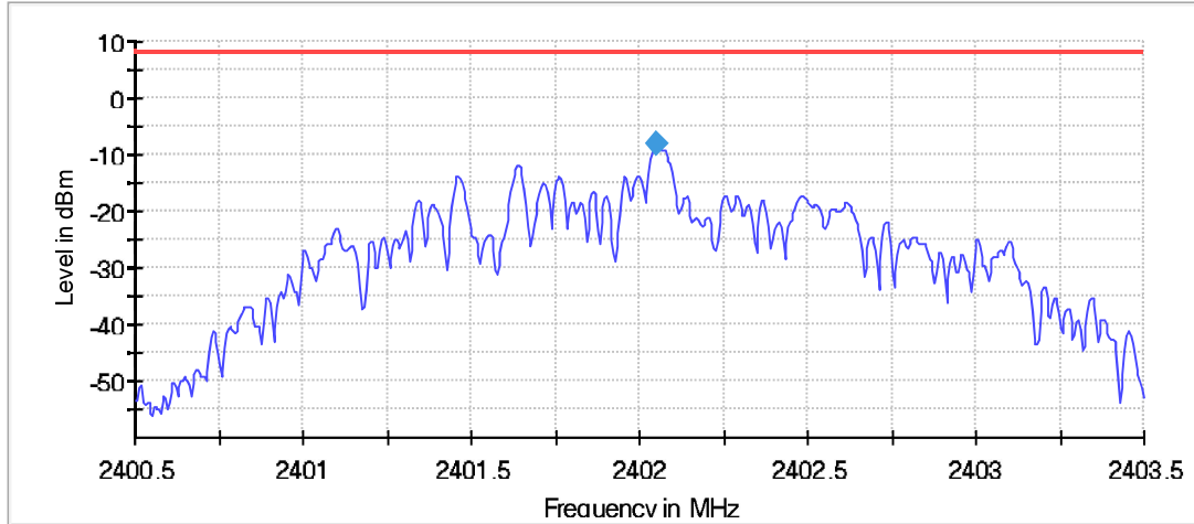
Peak Power Spectral Densitv
