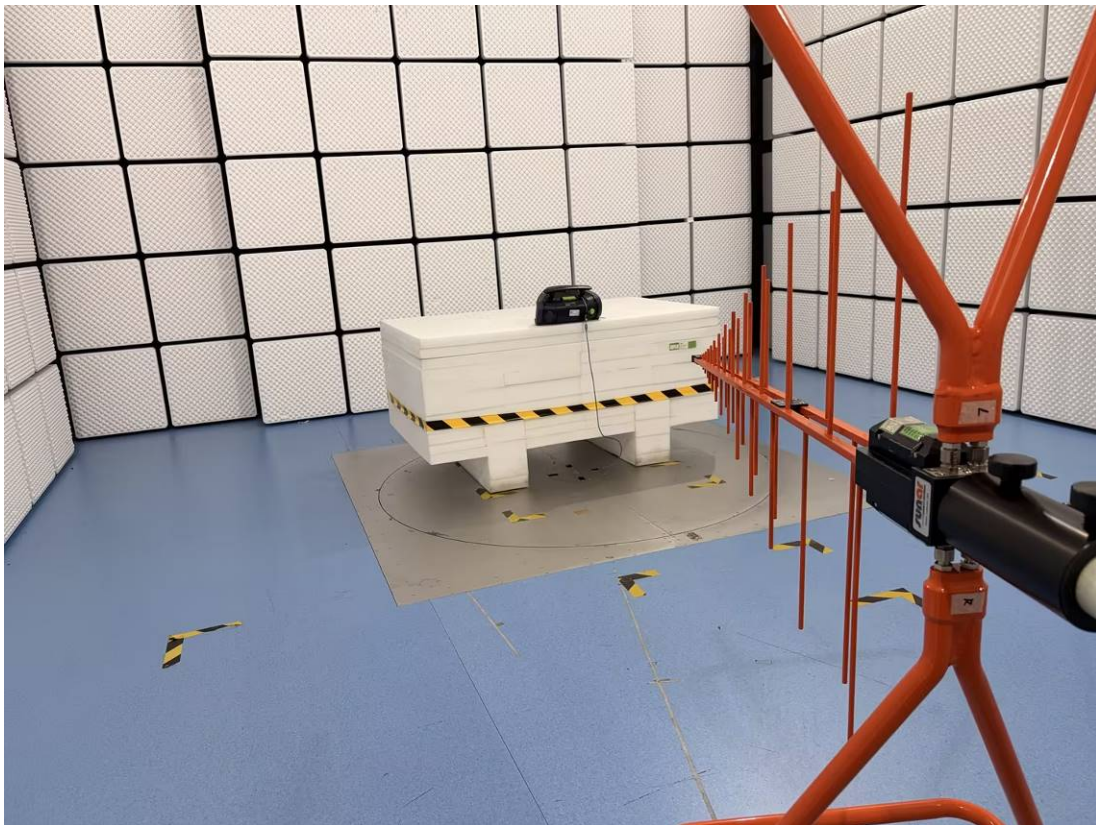
RE – Front View (30MHz~1GHz)_Powered by Battery(BP 18 Li 8,0 HP-ASI)
