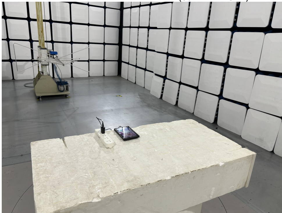
Photo of Radiation Emission Test (30MHz ~ 1GHz)
