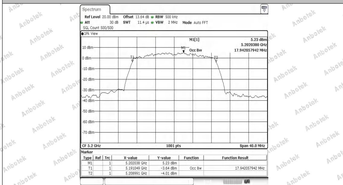
11N20SISO-Ant1-5200
