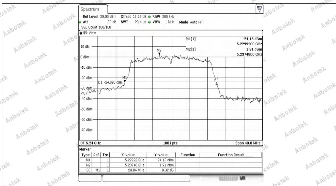
11N20SISO-Ant1-5240
