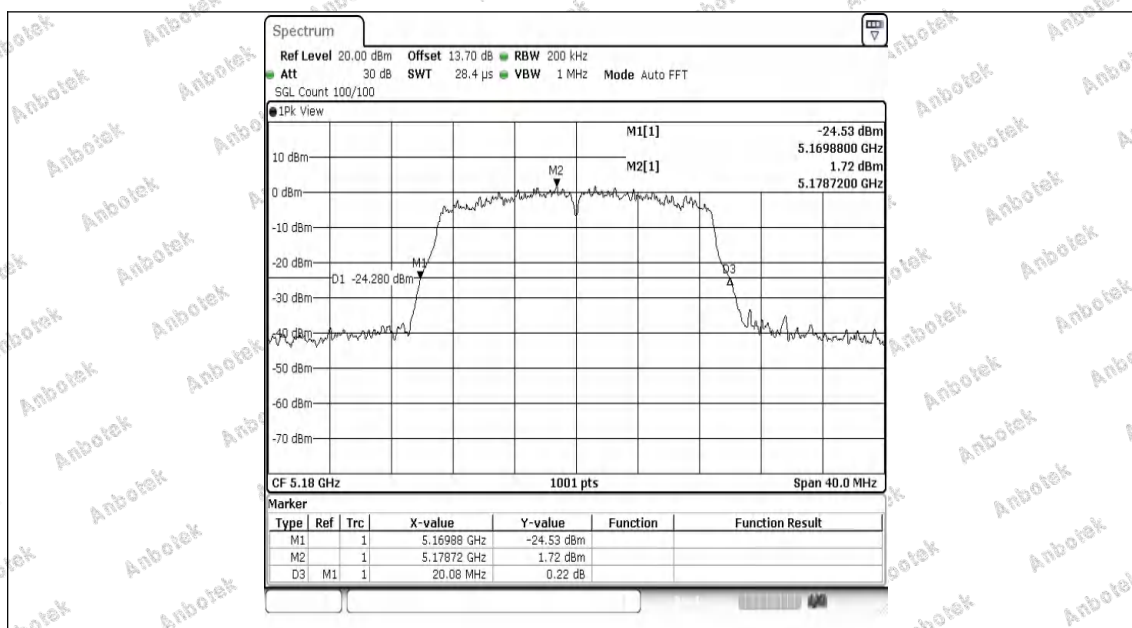
11AC20SISO-Ant1-5180
