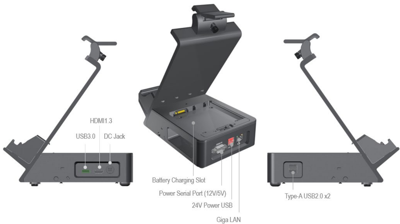
Figure7: Tegar TRT-3493-12 Docking Station Placement (without Cable Cover)
