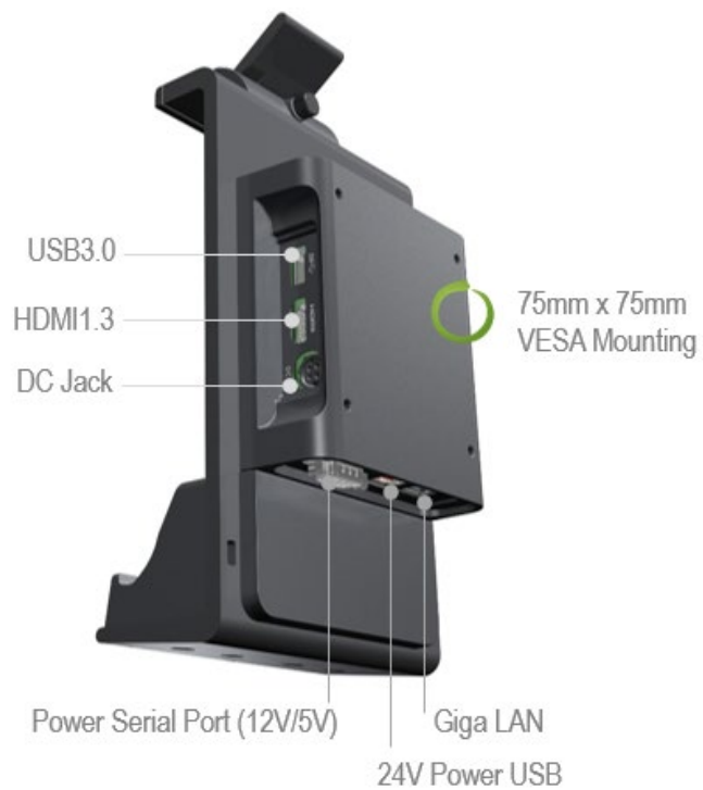
Figure9: Tegu TRT-3493-12 Extension Cover Placement
