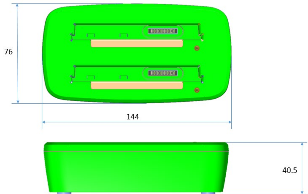
Figure5: Tegar TRT-3493-12 Battery Charger Dimension
