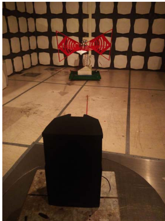
RE 30MHz-1GHz
