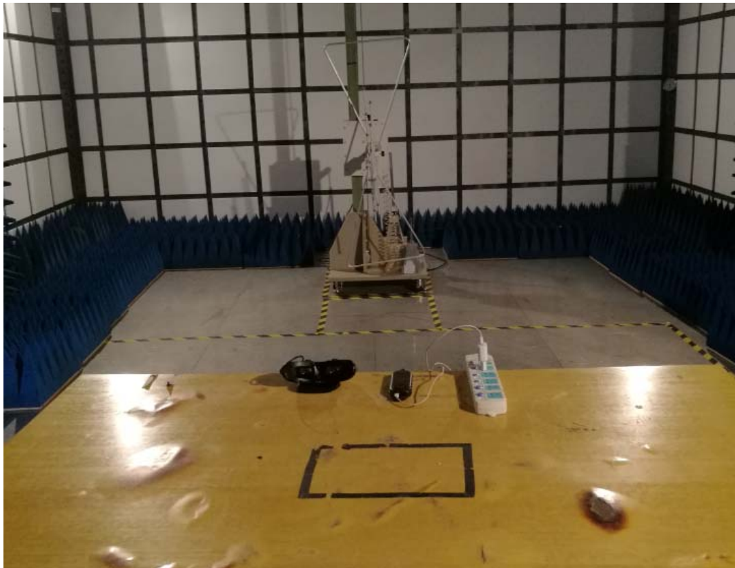
Radiated emission 30MHz~1GHz
