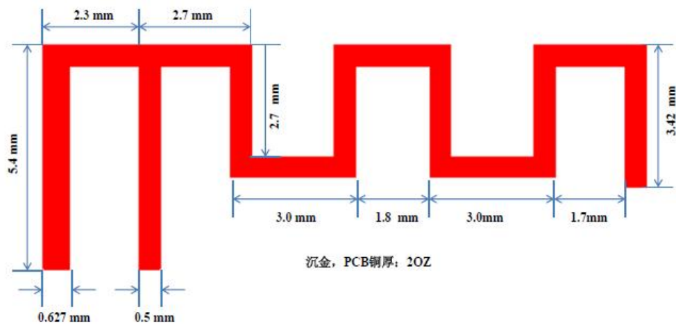
Antenna Dimension for GTAG
