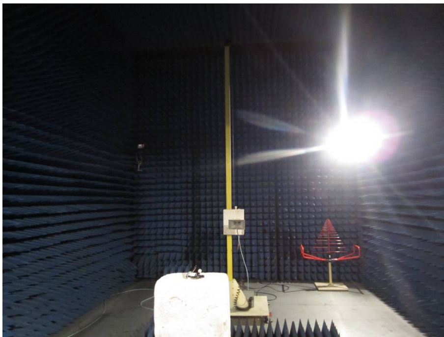
RADIATED EMISSION TEST SETUP (ABOVE 1 GHz) FROM 1.5M-HEIGHT TEST TABLE
