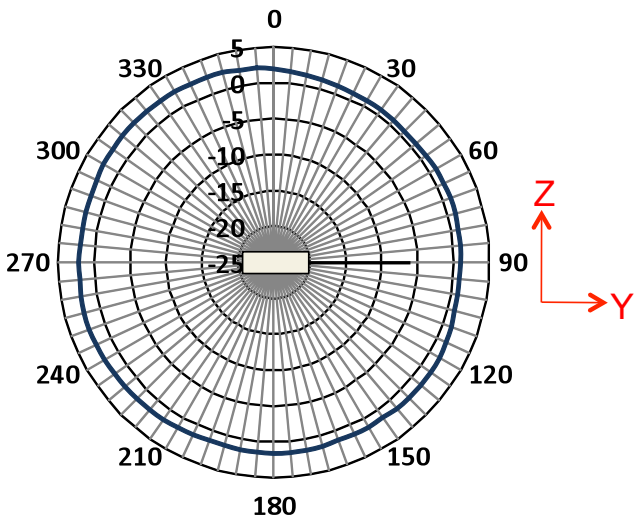
Figure 3d: Radiation diagram of Z-Y plane showing combined polarizations at 2.45 GHz
