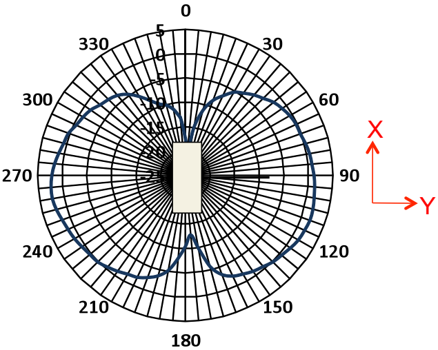
Figure 3b: Radiation diagram of X-Y plane showing combined polarizations at 2.45 GHz
