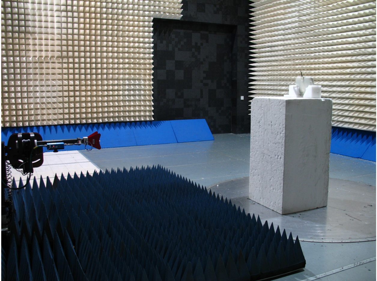
Radiated Emissions (transmitting)
