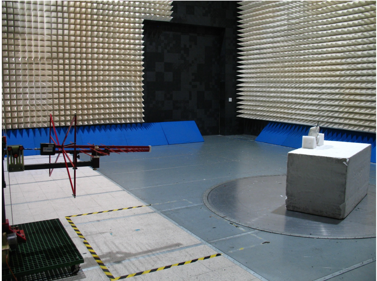
Radiated Emissions (idle)
