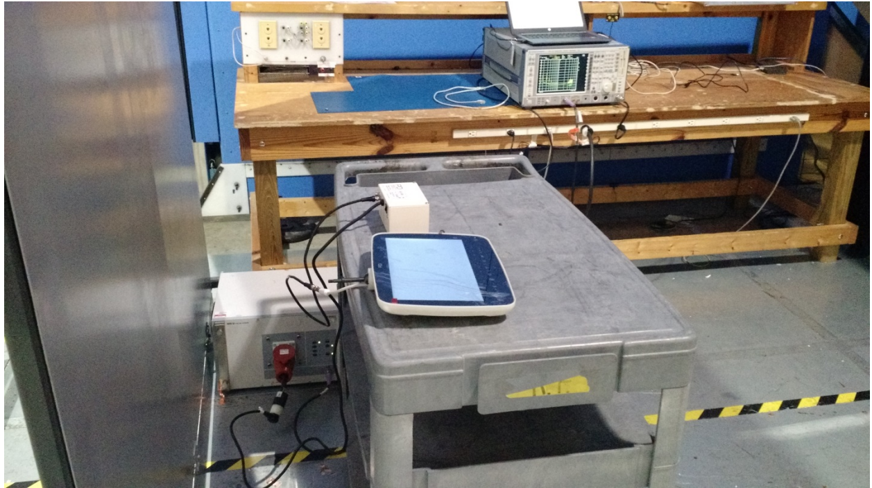
Conducted Emissions
