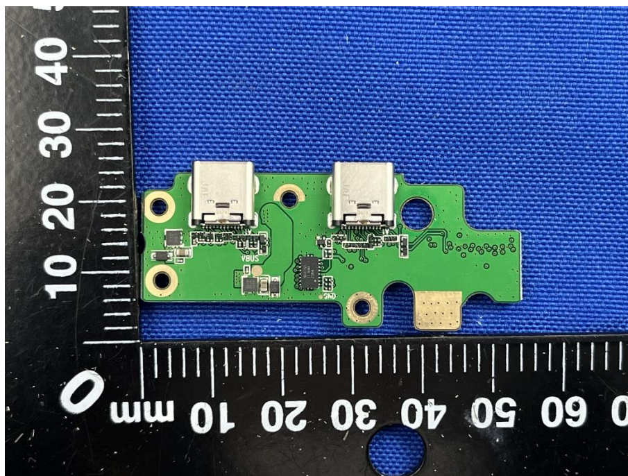
SUB BOARD 3 REAR VIEW
