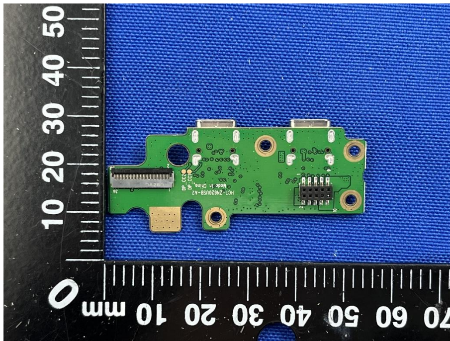
SUB BOARD 3 TOP VIEW
