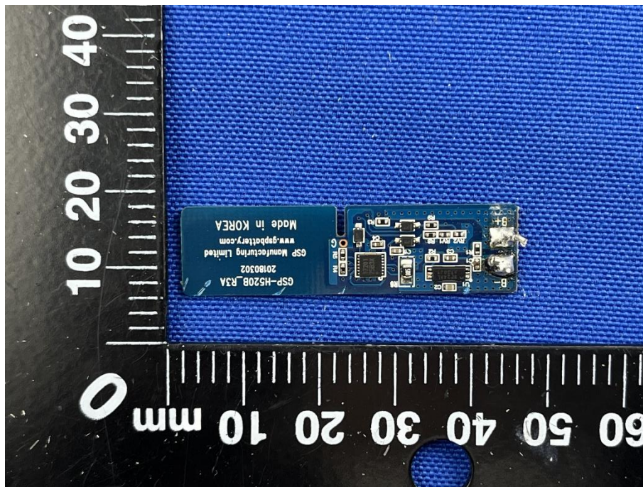
SUB BOARD 8 TOP VIEW
