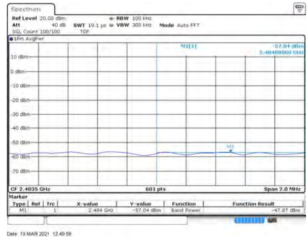
802.11g HIGH CHANNEL, Reference level
