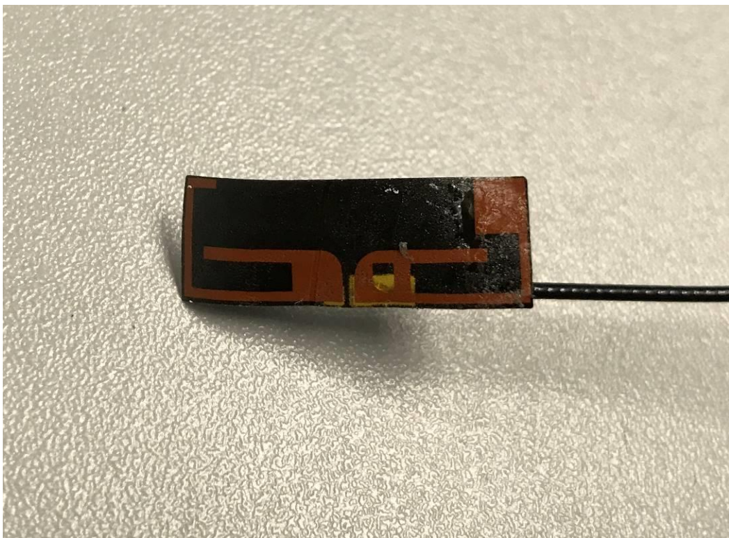
Internal View
