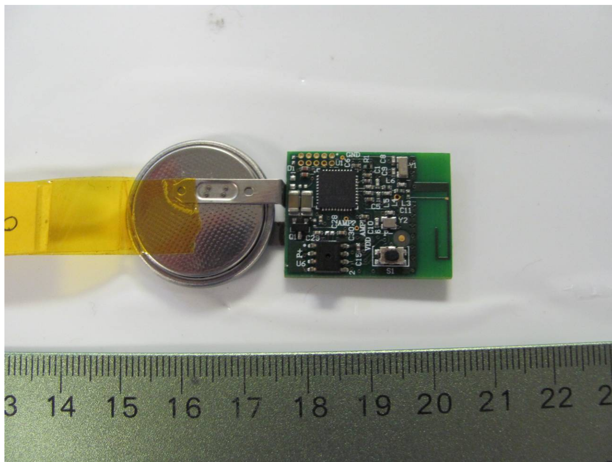
Figure 1. Component Side
