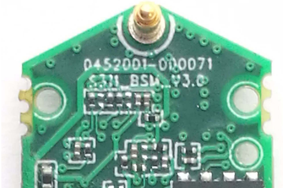
Part of PCB and exhibit the details of pogo pin connector
