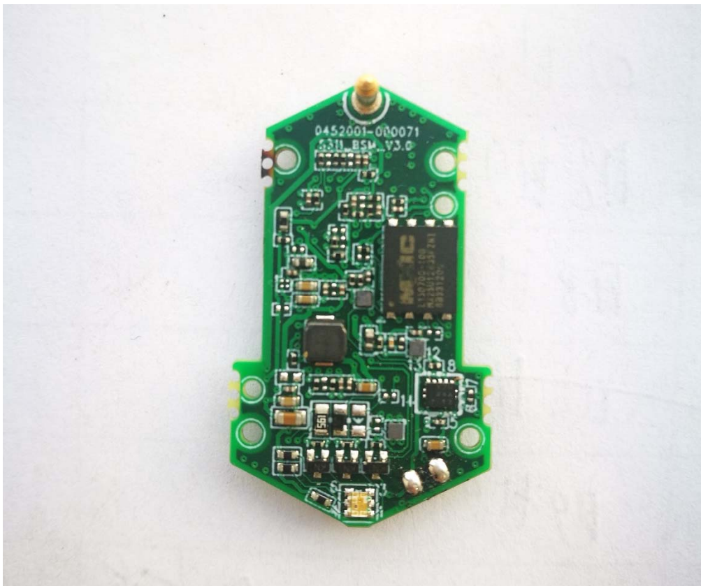
PCB with pogo pin connector
