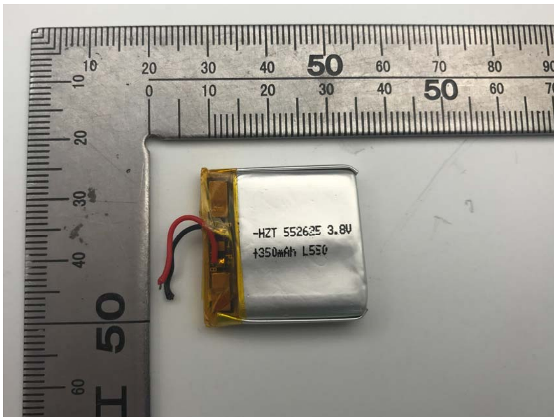
Battery View
