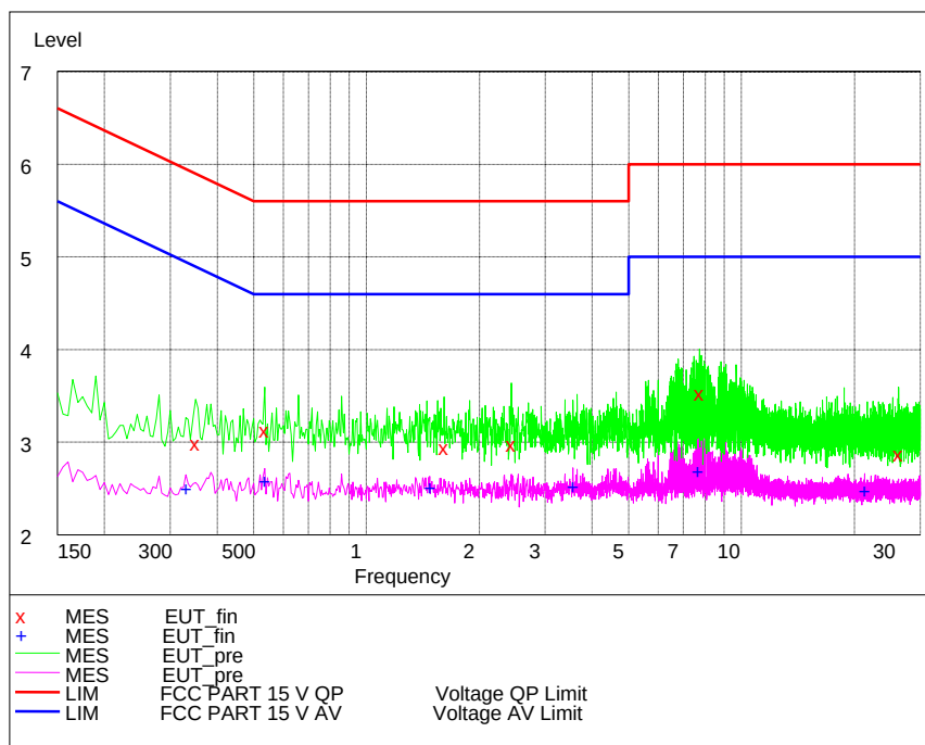
Conducted emission N Line
