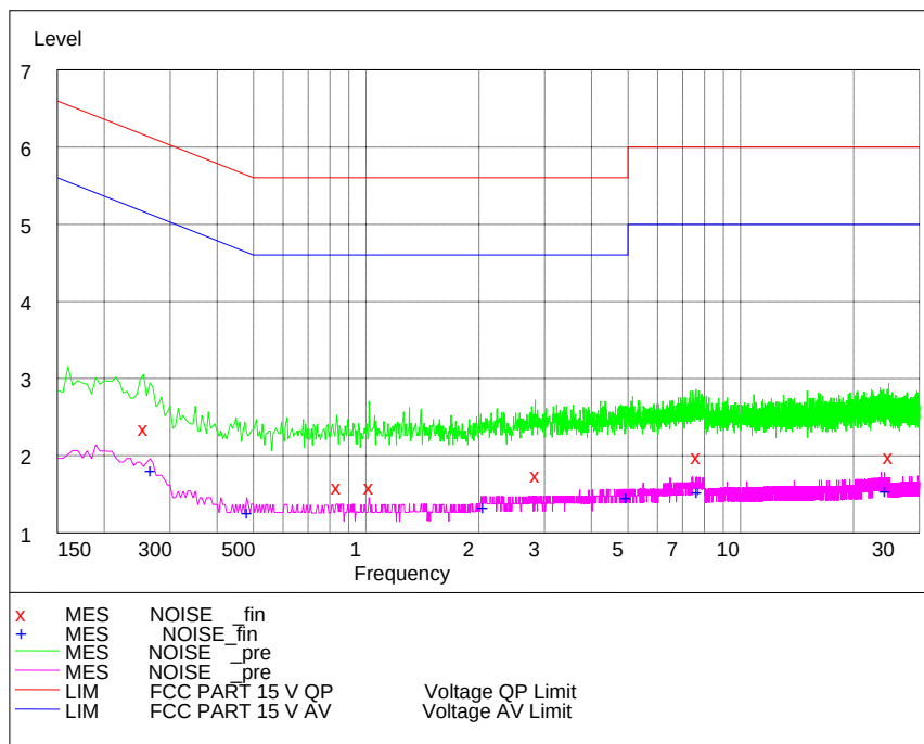
Conducted emission L and N Line
