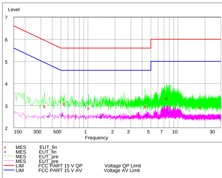
Conducted emission L Line
