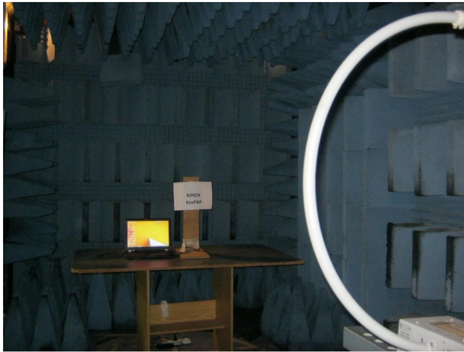
Radiated Emission Test for 0.009-30MHz
