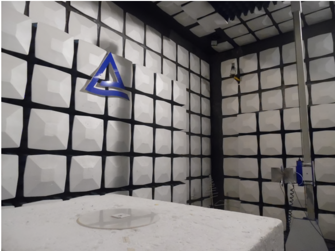
Photograph 4: Set-up for Radiated Spurious Emission, 18GHz - 26.5GHz
