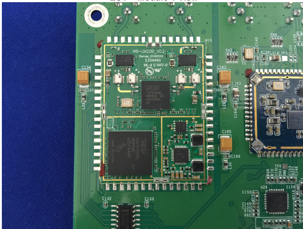
EUT – Module 1 View
