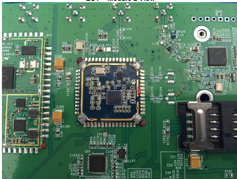
EUT – Module 2 View
