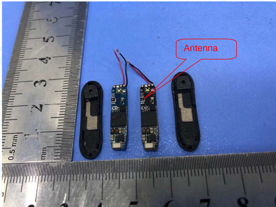
Photo 14 Appearance PCB
