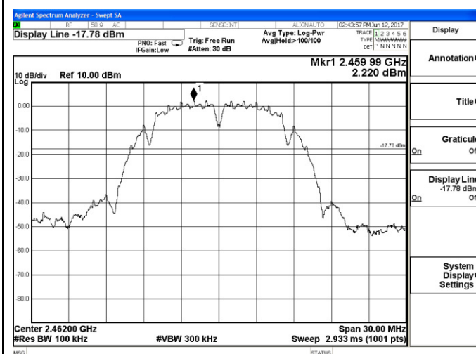
802.11b_High Channel
