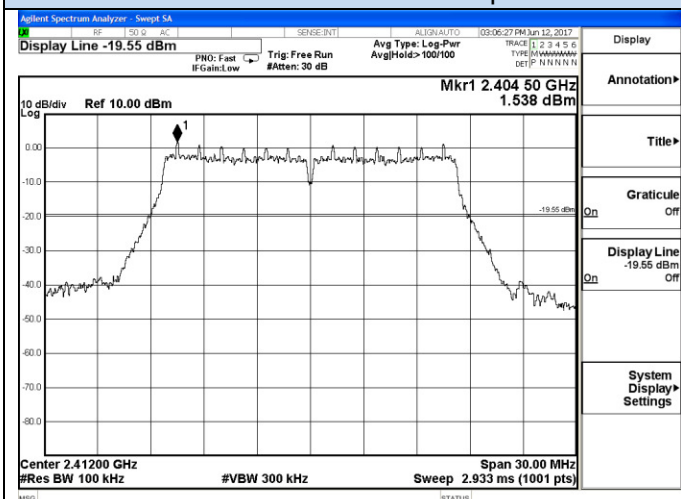
802.11g Low channel Reference
