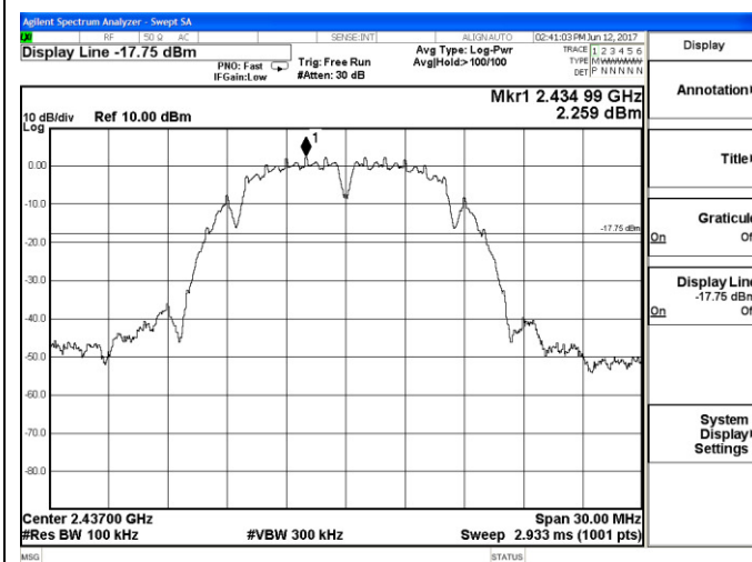
802.11b_Middle Channel
