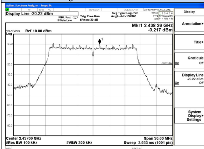
802.11g Middle channel Reference
