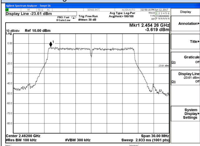
802.11g High channel Reference
