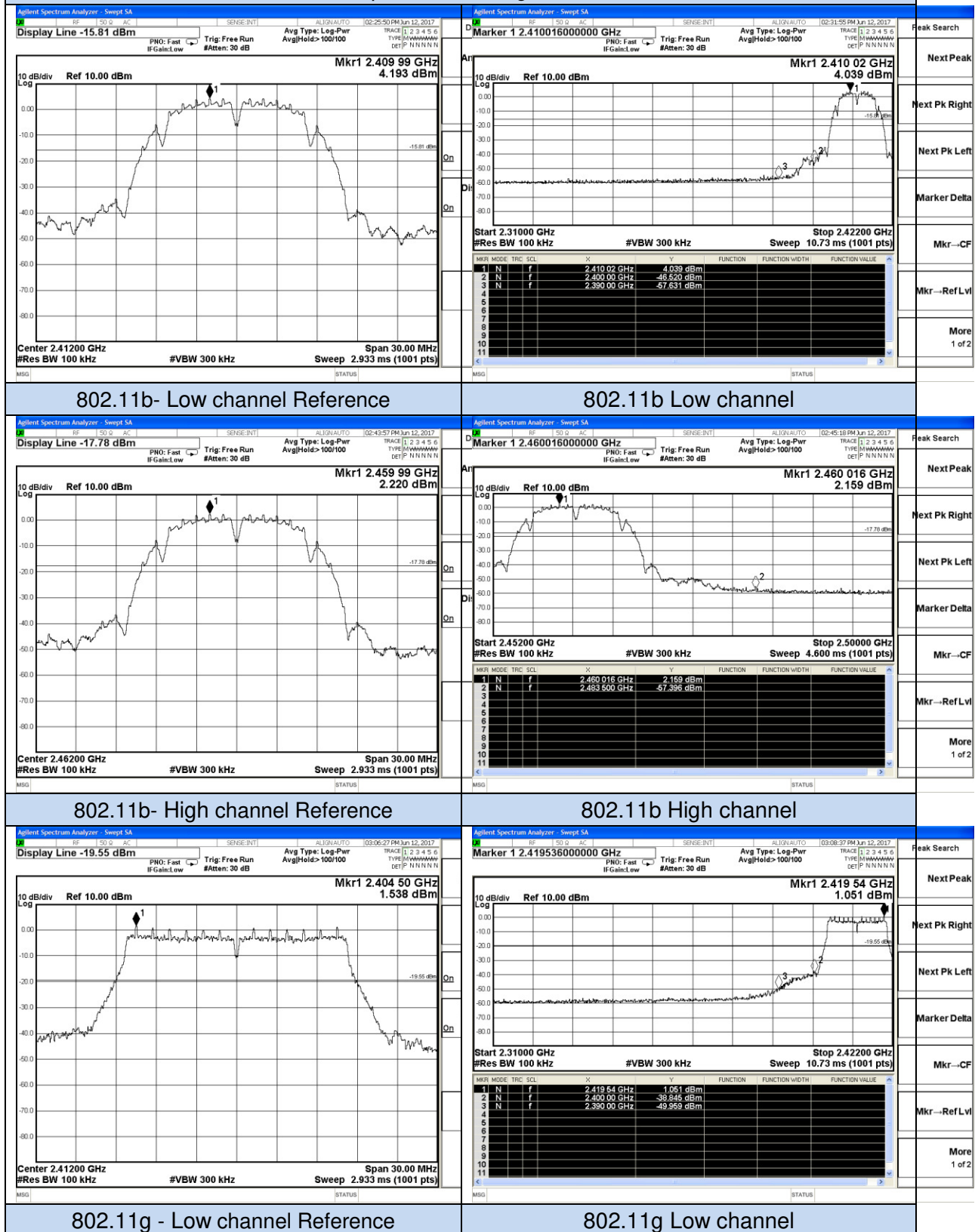
Test plot of Band Edges Test
