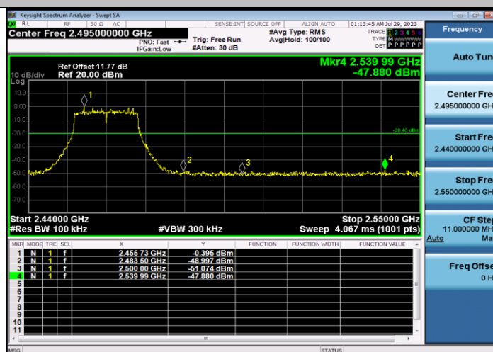
11N20SISO_Ant1_High_2462
