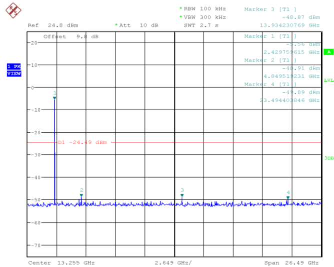
Plot 16. 1Mbps, 2402MHz 30MHz-26.5GHz Spurious
