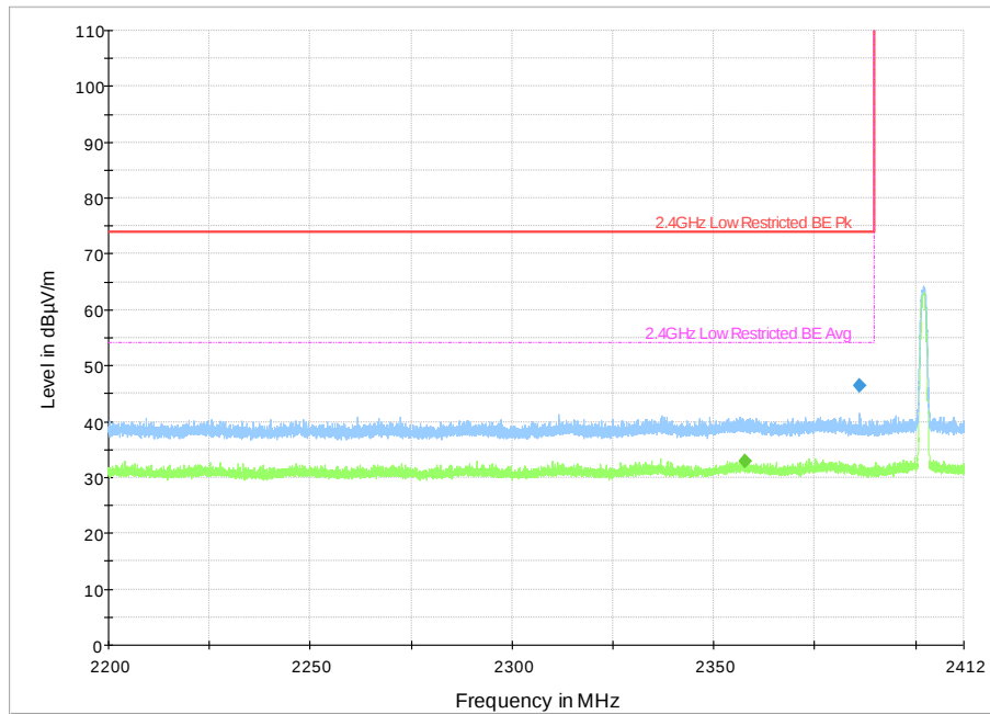
Plot 19. 1Mbps, 2402MHz, Lower Band Edge, Restricted
