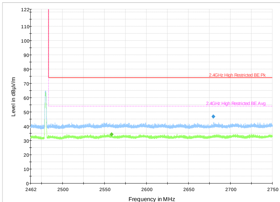
Plot 20. 1Mbps, 2480MHz, Upper Band Edge, Restricted
