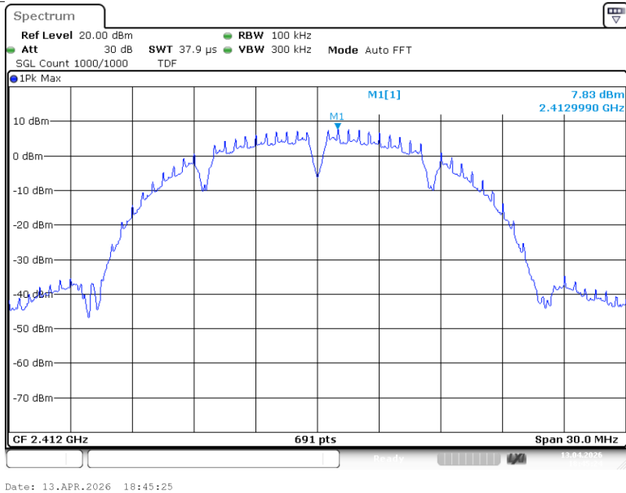
Tx. Spurious NVNT b 2412MHz Ant1 Ref
