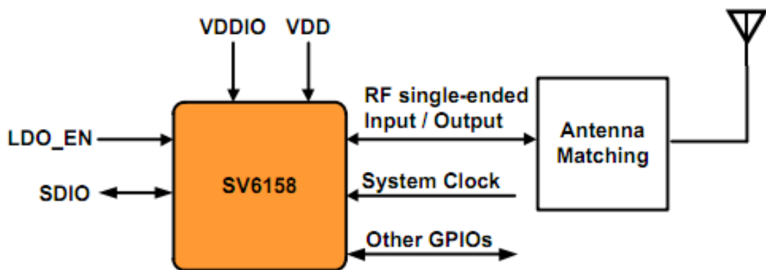
SV6158 System Block Diagram
